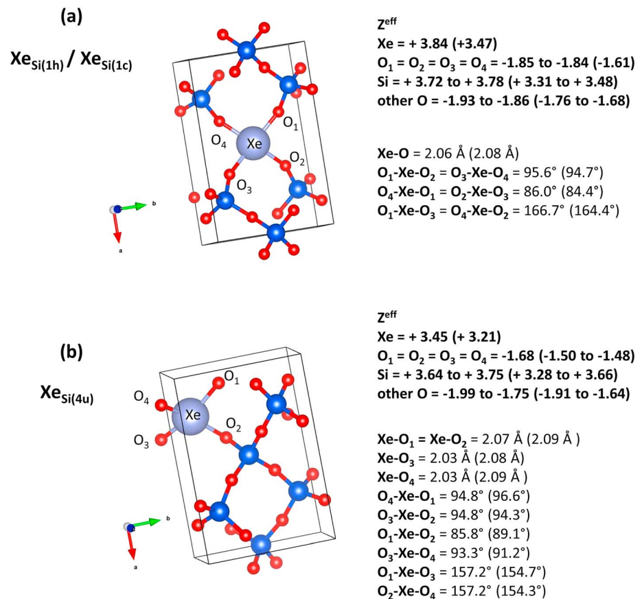
Figure 4. Relaxed structures of the new (Xe,Si)O 2 phase at 0 GPa with Xe in either 1h, 1c (a) or 4u (b) site. Bond lengths, angles and atomic charges ( Z^{\text{eff}} ) are given for 5.56 at% Xe and in brackets for 0.62 at% Xe. Si, O, and Xe are blue, red, and light blue ball, respectively.
