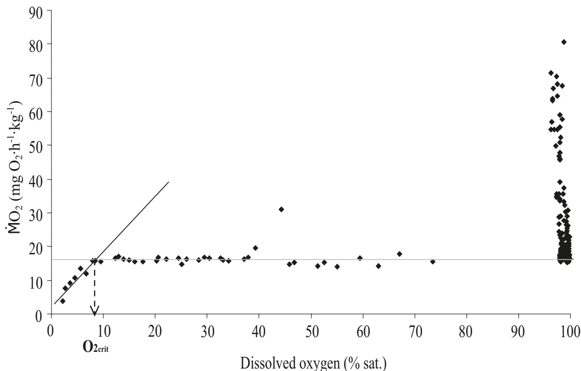
Fig. 1. Oxygen consumption ( \dot{M}_{O_2} , mg O 2 ·h -1 ·kg -1 ) as a function of dissolved oxygen (DO; % saturation) for an individual Greenland halibut. O_{2crit} is the intercept of the standard metabolic rate (SMR, grey line) and the regression line (black line) through the points below SMR. The scatter of points at 100% saturation correspond to data recorded during the 48 h prior to the gradual decrease in DO level and thus include values recorded during spontaneous activity of fish.
