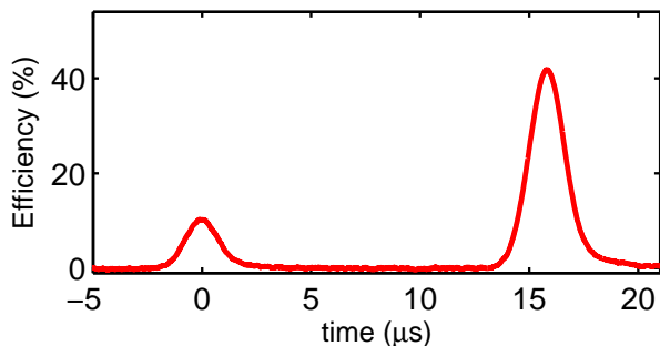
Fig. 2. ROSE echo for \alpha L = 2.3 . The first pulse is the transmitted signal. The echo is retrieved at 2t_{23} = 16\ \mu\text{s} with an efficiency of 42%.
