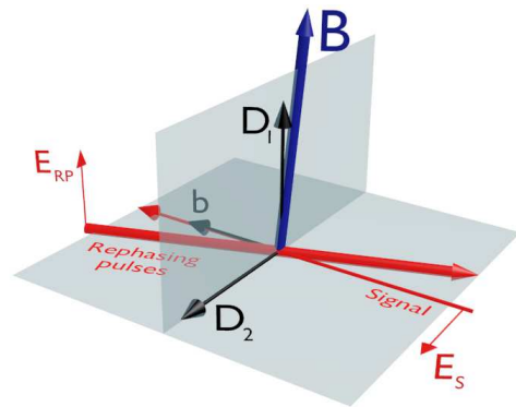
Fig. 1. Beams (signal and rephasing), polarizations (noted E_{\text{RP}} and E_{\text{S}} respectively) and magnetic field \vec{B} orientations. \mathbf{D}_1 , \mathbf{D}_2 and \mathbf{b} are the \text{Y}_2\text{SiO}_5 optical extinction axes.
