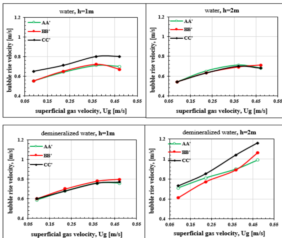
Figure 18. Relationship between bubble rise velocity and superficial gas velocity.
