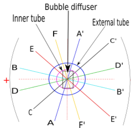
Figure 8. Schematic representation of the radial measurement axes by the optical bi-probe.
