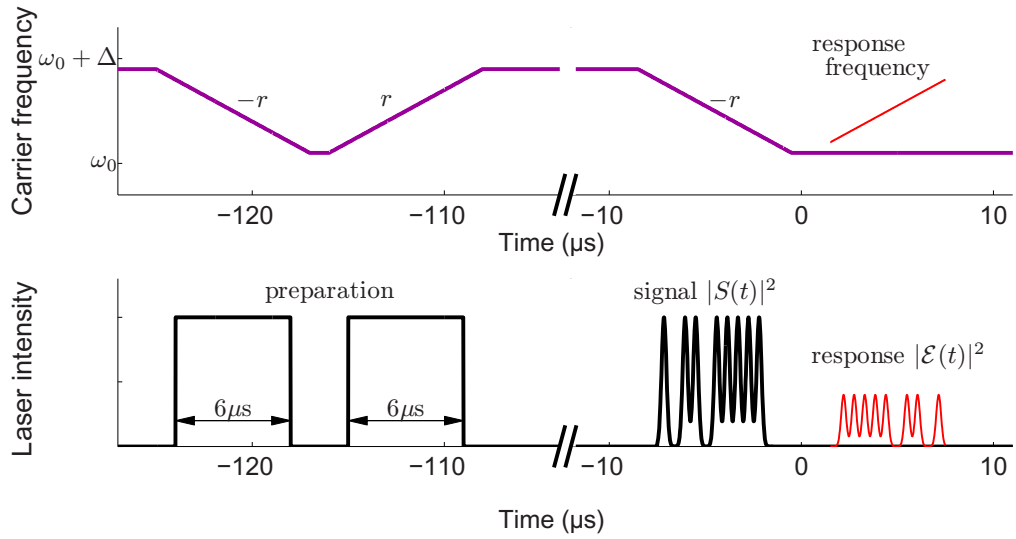
Figure 8. Experimental pulse sequence. Thick lines: incoming preparation and signal pulses. Thin line: dispersive filter first-order response, emitted as a chirp with rate r , carrying the time-reversed signal.
