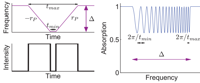
Figure 6. Two chirped pulses with opposite chirp rates -r_P and r_P induce a quasi-sinusoidal absorption grating with variable spacing.
