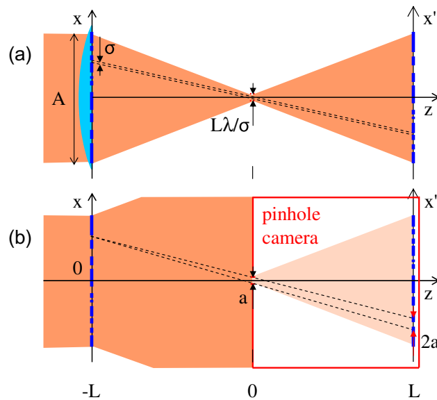
Figure 1. Conventional optics image reversal schemes. In the upper box (a), the object at z = -L is illuminated by a collimated beam. The size of the object's smallest detail is represented by \sigma . The lens, placed side-by-side with the object, concentrates the energy on a \lambda L/\sigma -wide bottleneck in the focal plane ( z = 0 ). The imaging spatial resolution on the screen at z = L , of order \sqrt{\lambda L} , is limited by the Fraunhofer condition. The lower box (b) represents the pinhole camera. The black dashed lines depict the camera impulse response. They represent geometrical rays that are traced from a single point on the object to the screen, through the a -wide slit. The shaded zones with different shade levels are intended to show that a small part of the incoming energy is allowed by the slit to the screen.
