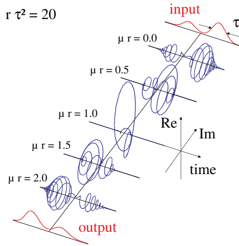
Figure 2. Approximate imaging for time reversal. Passing through a time lens, the incoming S(t) waveform is changed into S_{\mu=0}(t) = S(t) e^{irt^2/2} . Then S_{\mu}(t) propagates through a dispersive filter, from \mu = 0 at the input to \mu = 2/r at the output. The time variation of S_{\mu}(t) is displayed in 3D representation at different \mu -positions, illustrating the waveform compression into the focal plane, at \mu = 1/r , the subsequent stretching and the time reversal at \mu = 2/r . The phase evolution in the focal plane results from the time separation of the two incoming peaks. The output profile represents |S_{\mu=2/r}(t)| . In this simulation, r has been set equal to 20/\tau^2 , where \tau represents the full-width at half-maximum of the incoming peaks.
