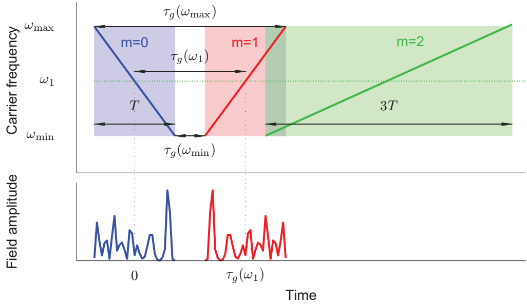
Figure 4. Carrier and signal time diagrams. The incoming carrier instantaneous frequency decreases with time from \omega_{\max} to \omega_{\min} . In contrast, the first-order response carrier frequency increases with time from \omega_{\min} to \omega_{\max} . The (\omega_{\min}, \omega_{\max}) interval is centered at \omega_1 . The outgoing response, centered at t = \tau_g(\omega_1) , is time reversed with respect to the incoming signal, centered at t = 0 . The carrier frequency range [\omega_{\min}, \omega_{\max}] and the signal duration T are connected by 2T = \tau_g(\omega_{\max}) - \tau_g(\omega_{\min}) . In the figure, the first- ( m = 1 ) and second- ( m = 2 ) order responses partly overlap. To avoid this, the signal duration must satisfy the condition T \leq \tau_g(\omega_1)/2 .
