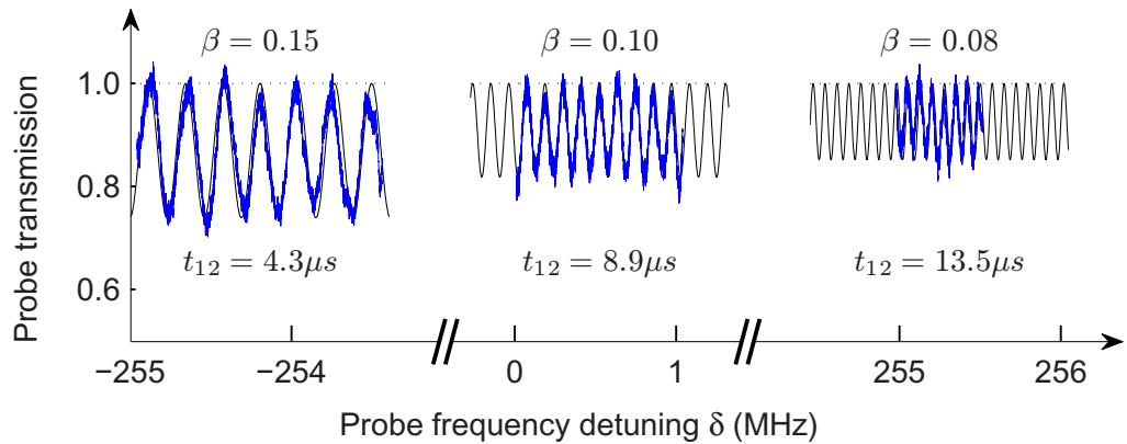
Figure 7. Normalized transmission measurement around different frequencies within the 1.09 GHz engraved frequency range (blue line). After the two programming pulses, a weak slowly chirped pulse is sent to the crystal and its transmitted intensity is monitored. Depending on the spectral range probed, one observes a locally sinusoidal modulation of the transmission, with frequency-dependent spectral period 1/t_{12} and contrast \beta . Thin black line: [1 + \beta \sin(2\pi \delta t_{12} + \theta)] / (1 + \beta) .
