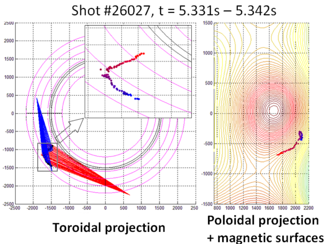
Fig. 3: (a) Toroidal projection and (b) poloidal projection of the trajectory of a dust particle experiencing a collision the ICR antenna limiter. First steps of the trajectory are depicted in blue and final steps in red (color online).
