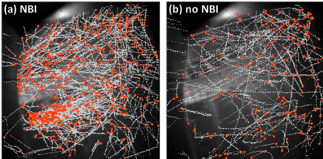
Fig. 6: (a) Dust trajectories reconstructed in 583 seconds of discharge with NBI as the only auxiliary heating system. Dust particles mostly move to the right. (b) Dust trajectories reconstructed during 1660 seconds of discharges without NBI. Dust particles mostly move to the left, i.e. towards sector 7. (color online)
