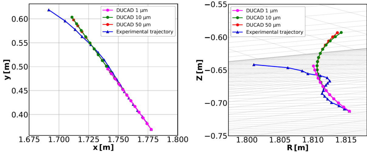
Fig. 4: Comparison between an experimental dust trajectory (solid blue line) and simulated trajectories for tungsten dust grains of three different radii: 1 micron (magenta), 10 microns (green) and 50 microns (red). Left picture shows projections of the trajectories in the toroidal view and right picture in the poloidal view. Markers show the dust positions at regular time interval, highlighting its acceleration in the last part of the trajectory (color online).
