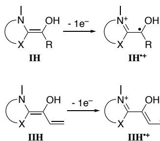
Scheme 2: Postulated Single Electron Transfer (SET) from Breslow intermediates of type IIH and IIH' . The corresponding radical intermediates IIH + and IIH'+ have been regarded as key intermediates in NHC-catalyzed radical reactions.
