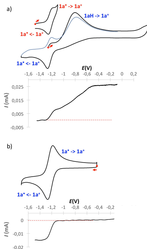
Figure 2: Cyclic voltammograms of a solution of 1aH with the impurity 1a• in \text{CH}_3\text{CN} + (\text{nBu})_4\text{NPF}_6 0.1 \text{ mol}\cdot\text{L}^{-1} (carbon electrode, \Phi = 3 mm; scan rate: 100 \text{ mV}\cdot\text{s}^{-1} ; E vs \text{Fc}/\text{Fc}^+ ) before (a) and after (b) quantitative electrolysis at -0.1 V and the corresponding rotating disk electrode voltammetry studies (RDE; 600 rpm; scan rate: 5 \text{ mV}\cdot\text{s}^{-1} ).
