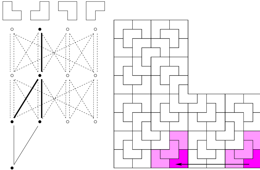
Figure 2: A doubly pointed pattern associated with a horizontal arrow h \in \mathcal{H}_{tr,3} . The arrow represents the vector r_h . Here n = 2 (the paths have lengths 2), and n_h = 1 (the paths join further down at level n + n_h = 3 ).
