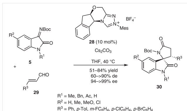
Scheme 7 NHC-catalyzed domino addition/cyclization reaction of isatin imines with \alpha,\beta -unsaturated aldehydes
