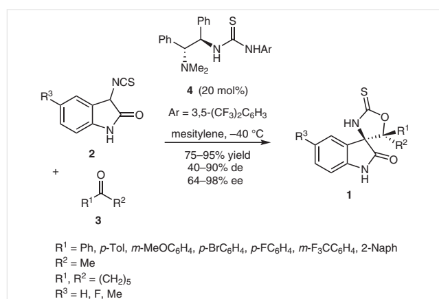
Scheme 1 Domino aldol/cyclization reaction of 3-isothiocyanato-2-oxindoles with ketones catalyzed by a thiourea
