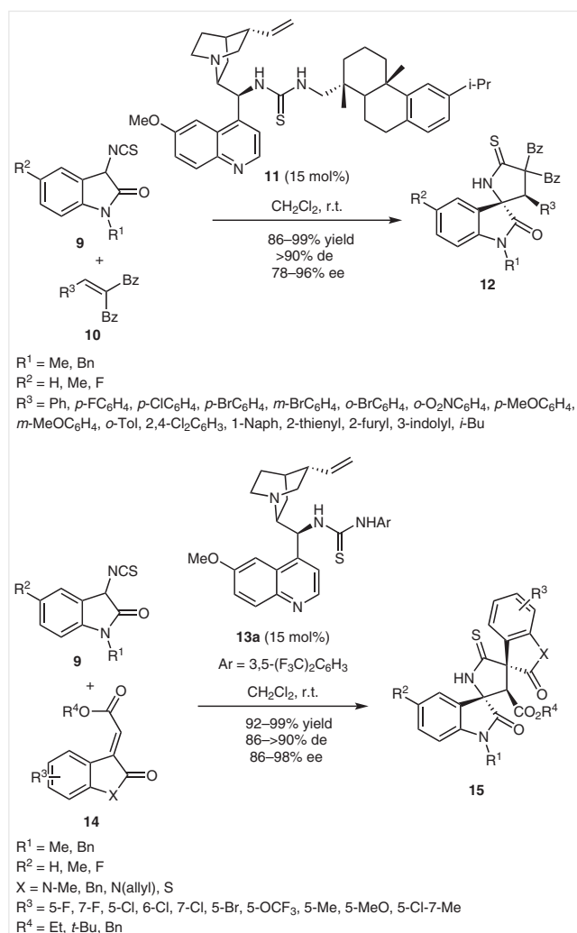
Scheme 3 Domino Michael/cyclization reactions of 3-isothiocyanato-2-oxindoles with electron-deficient alkenes and 3-methylene-2-oxindoles catalyzed by cinchona alkaloid derived thioureas
