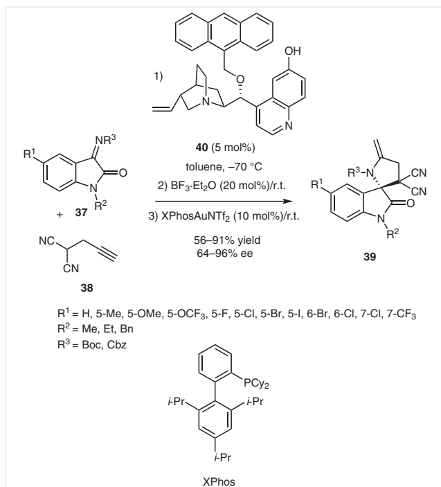
Scheme 10 Tandem multicyclic Mannich/hydroamination reaction of isatin imines with a propargylated malononitrile
