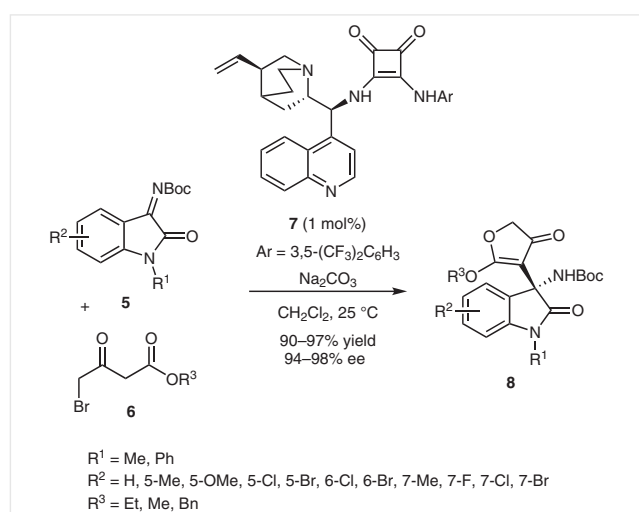
Scheme 2 Domino Mannich/cyclization reaction of isatin imines with 4-bromo-3-oxobutanoates catalyzed by a cinchona alkaloid-derived squaramide
