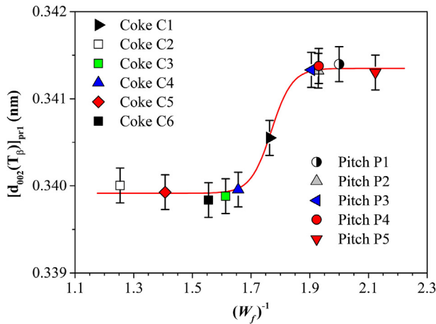
Fig. 15. Comparison between the experimental measurements of d_{002}(T_\beta) of Tables 3 and 4 and the results of Eq. (32) (where S_1 = 0.0014 nm, B_1 = 50 , d_{002}(T_\beta)_{min} = 0.3399 nm, W_c = 0.57 ) as a function of W_f ( 0.45 < W_f < 0.85 ) for the misorientation class G7( pr_1 ). The operating parameters of the heat treatment process to obtain this data ( pr_1 process) are HR_1 \sim 4^\circ \text{Cmin}^{-1} and t_{hold,1} = 10 min. T_\beta was arbitrarily defined as 2400 K in Section 2.3. The experimental error [65] on d_{002}(T_\beta) measurements is, at best, 2 \times 10^{-4} nm. (A colour version of this figure can be viewed online.)
