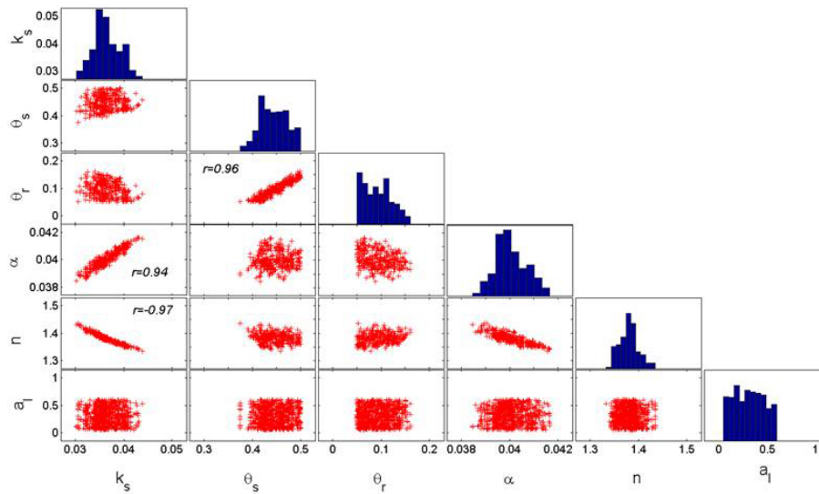
Figure 2. MCMC solutions for the transport scenario 1. The diagonal plots represent the inferred posterior probability distribution of the model parameters. The off-diagonal scatterplots represent the pairwise correlations in the MCMC drawing.
