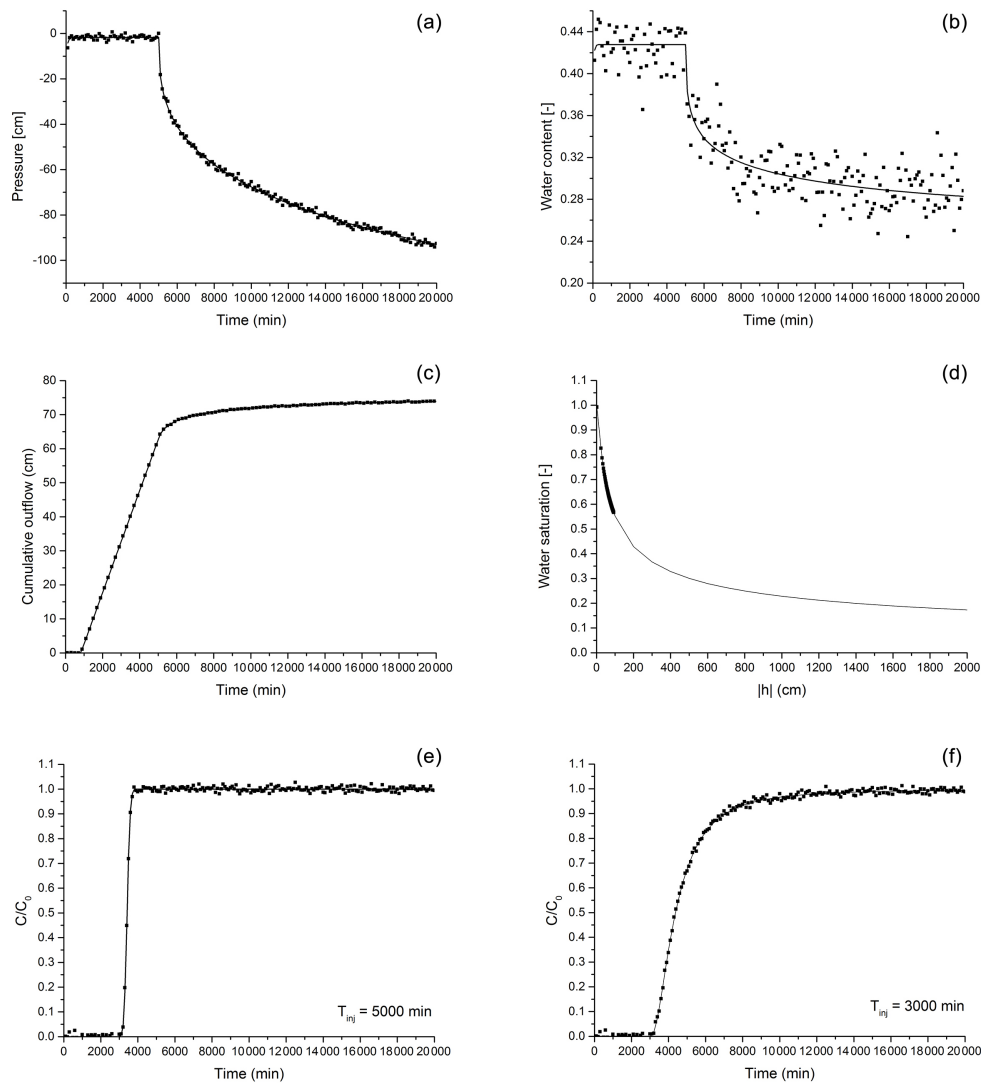
Figure 1. (a) Pressure head at 5 cm below the soil surface, (b) water content at 5 cm below the soil surface, (c) cumulative outflow, (d) retention curve, (e) output concentration for T_{inj} = 5000 and (f) for T_{inj} = 3000 min. Solid lines represent model outputs and dots represent the sets of perturbed data serving as conditioning information for model calibration.
