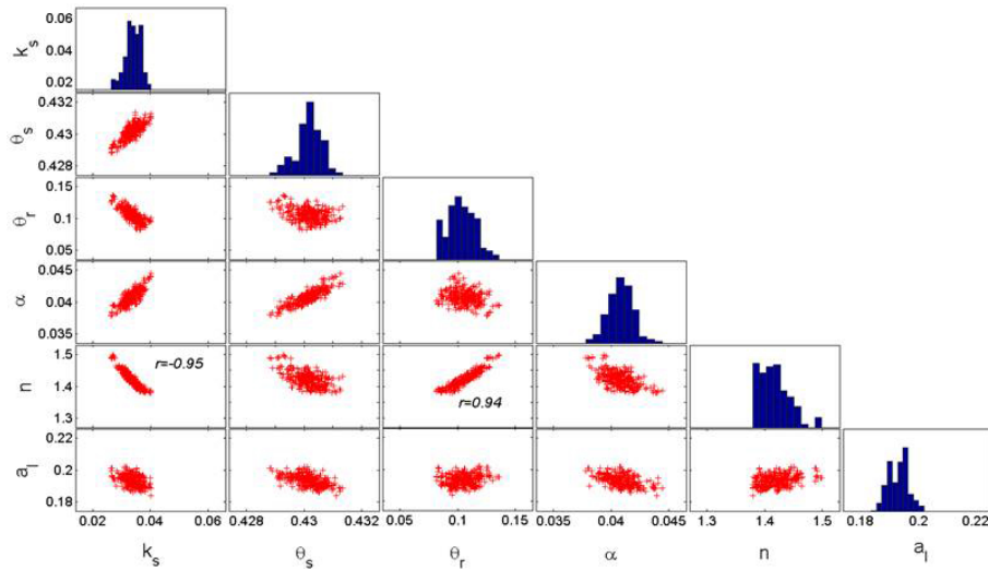
Figure 8. MCMC solutions for transport scenario 7 (see Fig. 2 caption).
