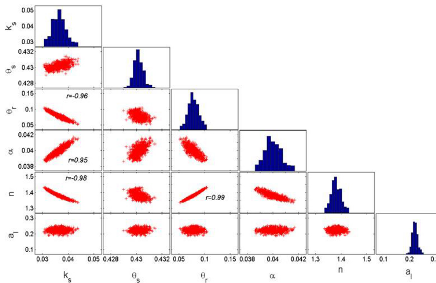
Figure 5. MCMC solutions for transport scenario 4 (see Fig. 2 caption).
