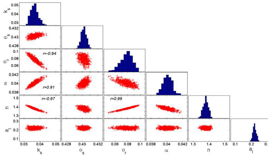
Figure 4. MCMC solutions for transport scenario 3 (see Fig. 2 caption).
