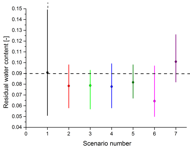
Figure 11. Posterior mean values and 95 % confidence intervals of the residual water content for the different scenarios.
