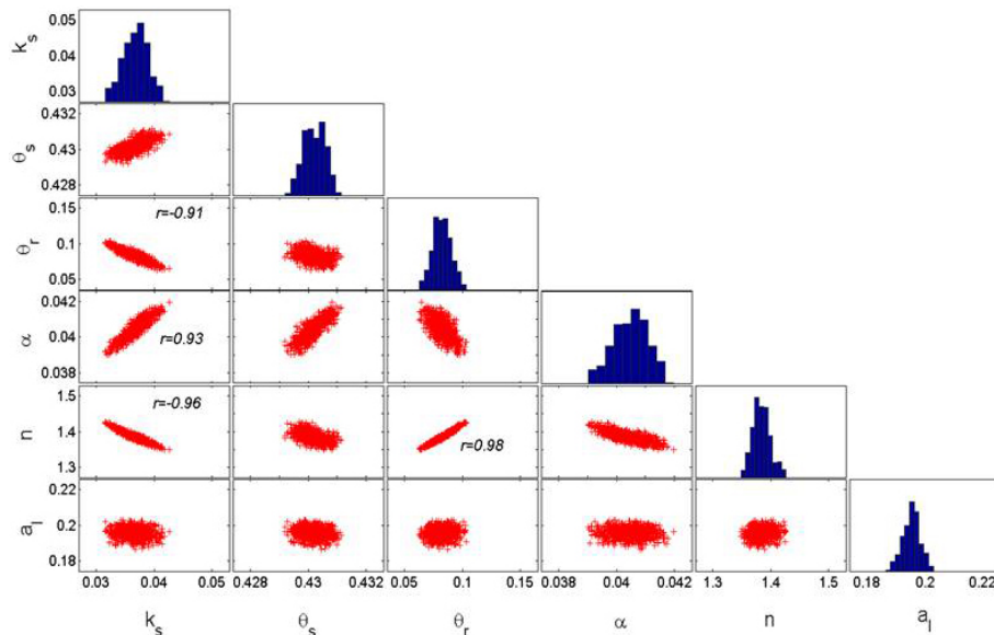
Figure 6. MCMC solutions for transport scenario 5 (see Fig. 2 caption).
