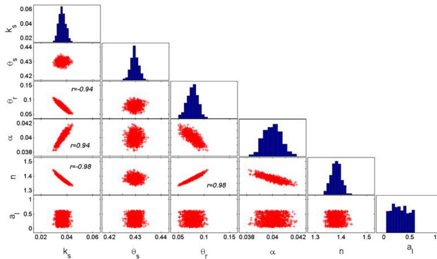
Figure 3. MCMC solutions for transport scenario 2 (see Fig. 2 caption).
