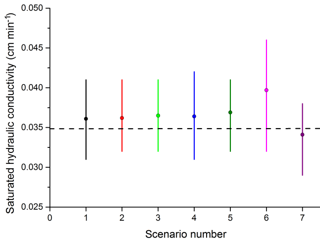
Figure 9. Posterior mean values and 95 % confidence intervals of the saturated hydraulic conductivity for the different scenarios.
