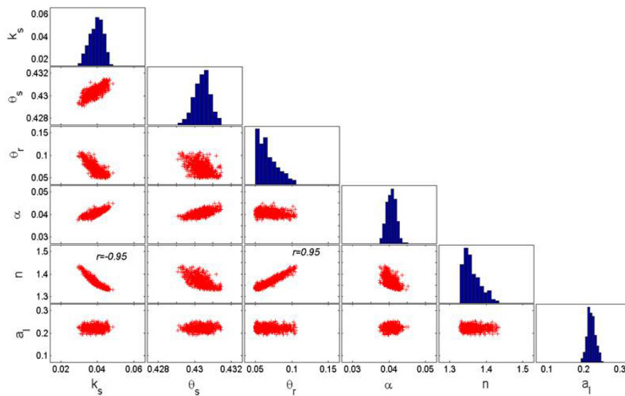
Figure 7. MCMC solutions for transport scenario 6 (see Fig. 2 caption).
