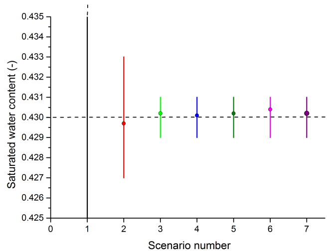
Figure 10. Posterior mean values and 95 % confidence intervals of the saturated water content for the different scenarios.
