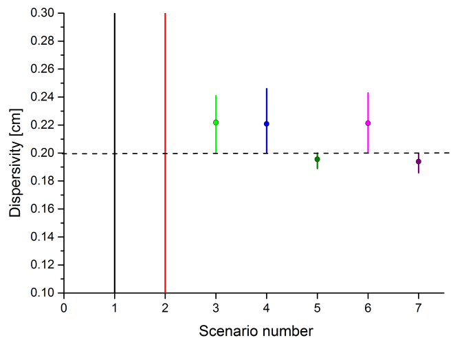
Figure 14. Posterior mean values and 95 % confidence intervals of dispersivity for the different scenarios.
