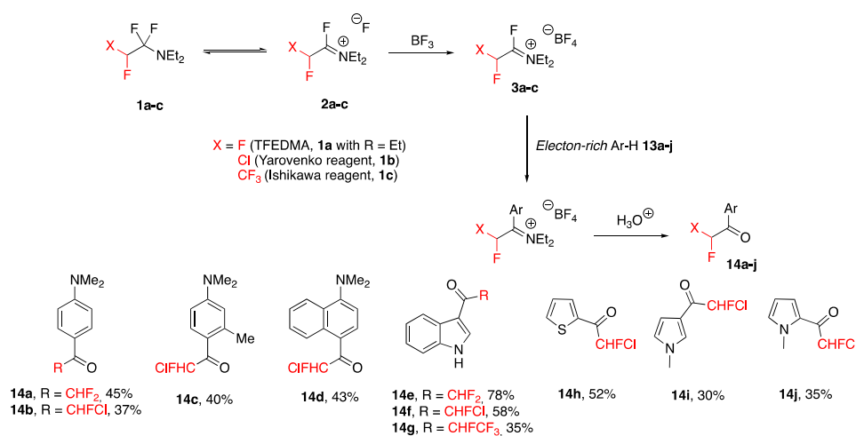
Scheme 7. Acylation of electron-rich aromatics with FARs by Wakselman et al. [66].
