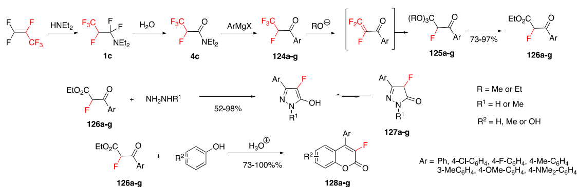
Scheme 32. Synthesis of fluorinated heterocycles from the hydrolyzed Ishikawa reagent [106].
