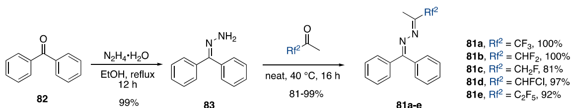
Scheme 20. Preparation of fluoroacetone-derived azines from benzophenone hydrazone.
