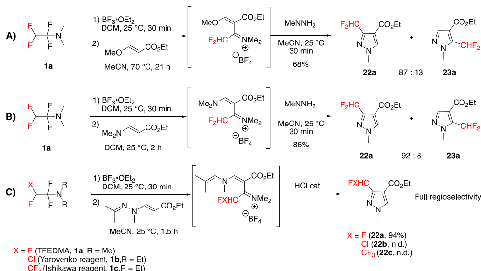
Scheme 12. Use of FARs ((A) Reaction of TFEDMA with methoxy acrylate; (B) with dimethylamino acrylate; (C) with a methylhydrazone) and acrylates to prepare ethyl 3-(difluoromethyl)-1-methyl-1H-pyrazole-4-carboxylate (DFMMP) with full regioselectivity.
