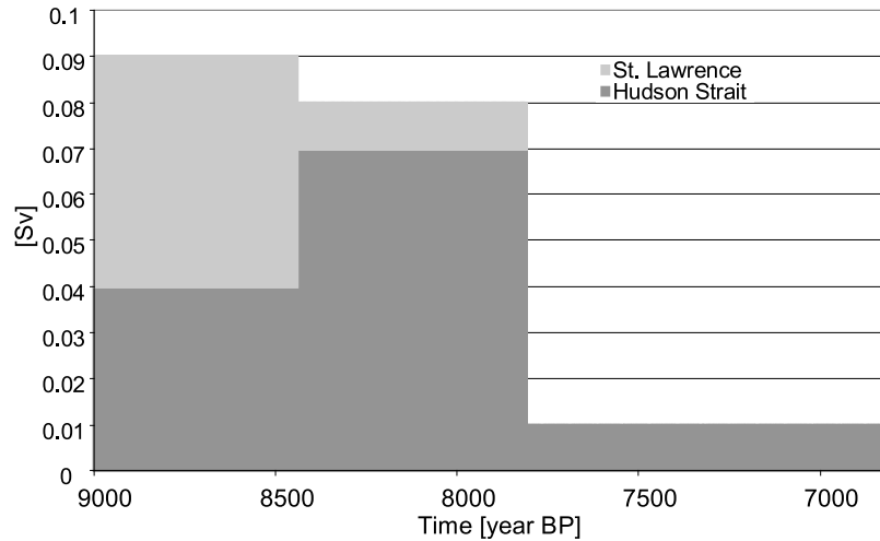
Figure 3. Applied background freshwater forcing (in Sv = 10^6 m^3 s^{-1} ), representing the LIS background melt rate, introduced in the St. Lawrence outlet and Hudson Strait in experiments OGMELT and OGMELTICE. This forcing is adjusted from Licciardi et al. [1999].
