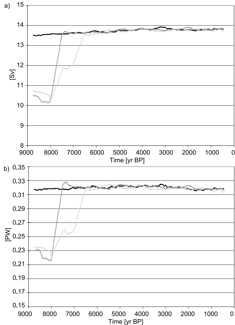
Figure 9. (a) Simulated export of NADW and (b) northward heat transport by the Atlantic Ocean at 20°S. Shown are the results of ORBGHG (black), OGMELT (dark gray), and OGMELTICE (light gray) as 499 year running means.
