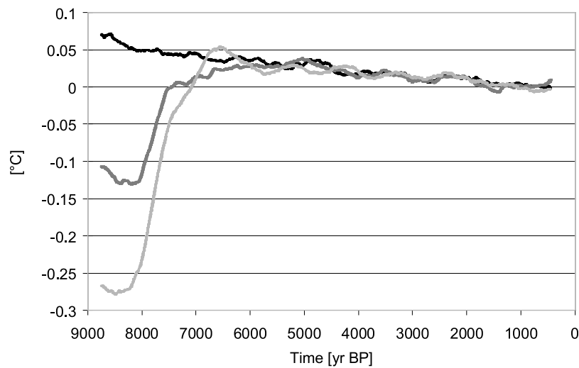
Figure 4. Simulated annual global SST anomaly ( ^\circ C ) relative to the preindustrial mean. Shown are the results for ORBGHG (black), OGMELT (dark gray), and OGMELTICE (light gray). A 499 year running mean was applied.
