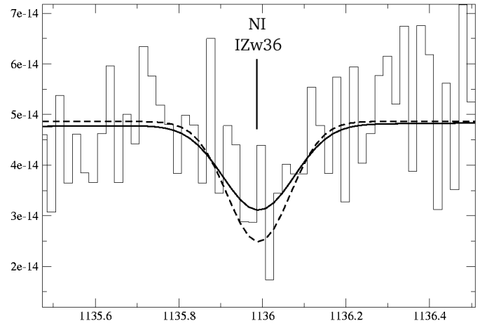
Fig. 5. Fit of the \lambda 1134.98 line. Data are binned by a factor 2 for display purposes. The solid line is for \log(\text{N I}/\text{H I}) = -6.88 and shows our best fit. The dashed line is for \log(\text{N I}/\text{H I}) = -5.63 and does not fit well the data.
