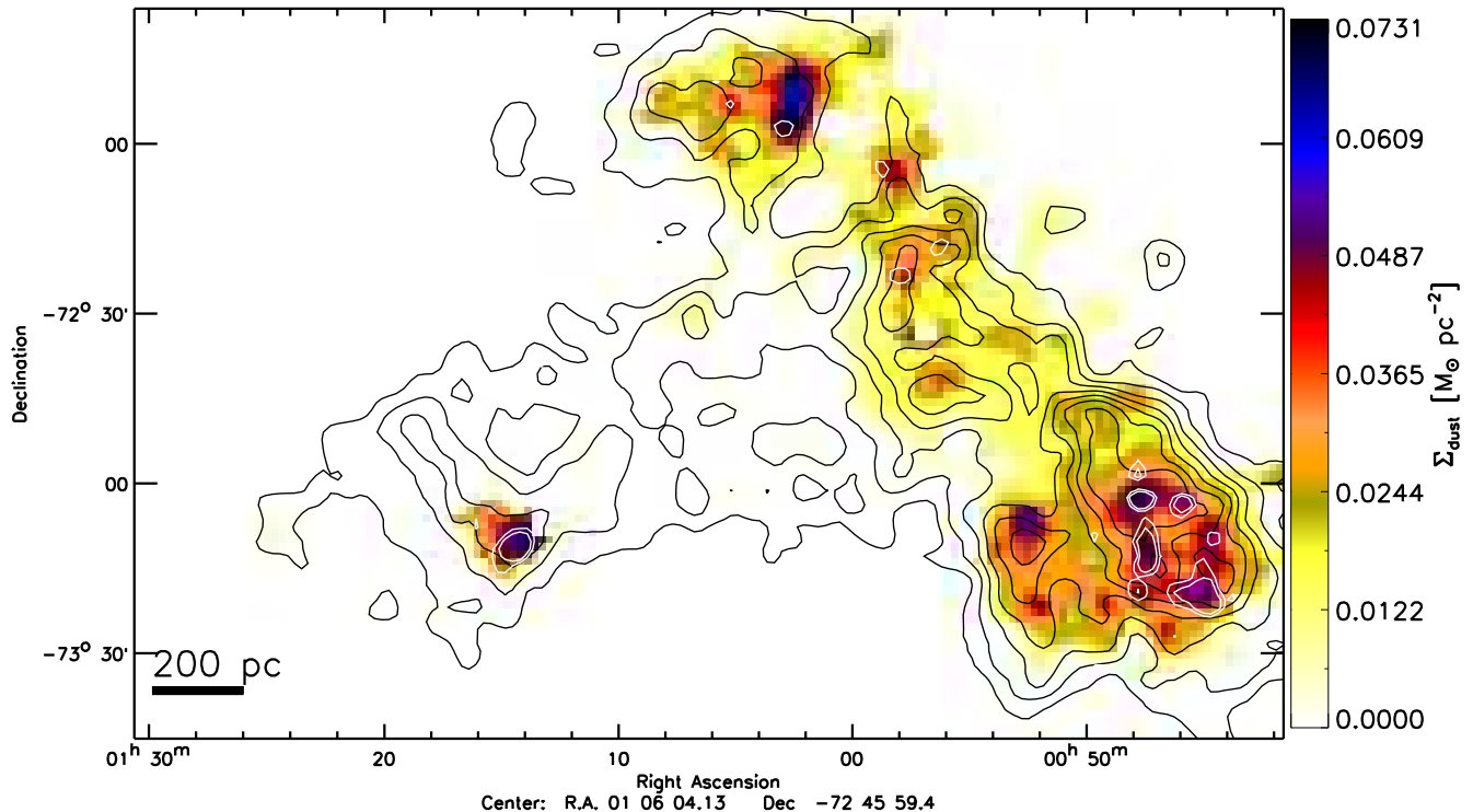
FIG. 2.— Map of the dust surface density in the SMC from Paper I at 2.6' ( 45 pc) resolution. The black contours show the H I surface density (Stanimirovic et al. 1999), with levels 40 - 100 M_{\odot} \text{pc}^{-2} in steps of 10 M_{\odot} \text{pc}^{-2} . The white contours show the CO integrated intensity (Mizuno et al. 2001a), with levels 0.5 and 0.8 \text{ K km s}^{-1} . Note that the color scale is different from Figure 1 due to the lower dust abundance in the SMC.
