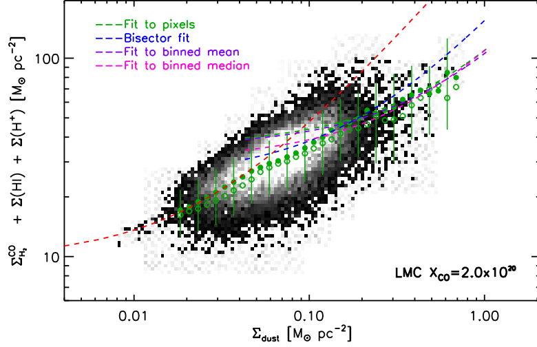
FIG. 11.— Pixel-to-pixel correlation between dust and total gas surface densities in the dense phase (CO detected) of the LMC, assuming values X_{\text{CO}}^{\text{fid}} . The distribution, shown by the grey scale, only includes pixels with CO detections. The green filled and empty circles correspond to the binned mean and median (as in Figures 5). Over-plotted are different linear fits. Our fiducial method, which consists in performing a \chi^2 minimization of the pixels to a linear function, is shown as a green dashed line. We also performed a bisector fit (blue), a linear fit to the binned mean (pink), and a linear fit to the binned median (purple). The resulting dust-gas slopes are summarized in Table 4.
