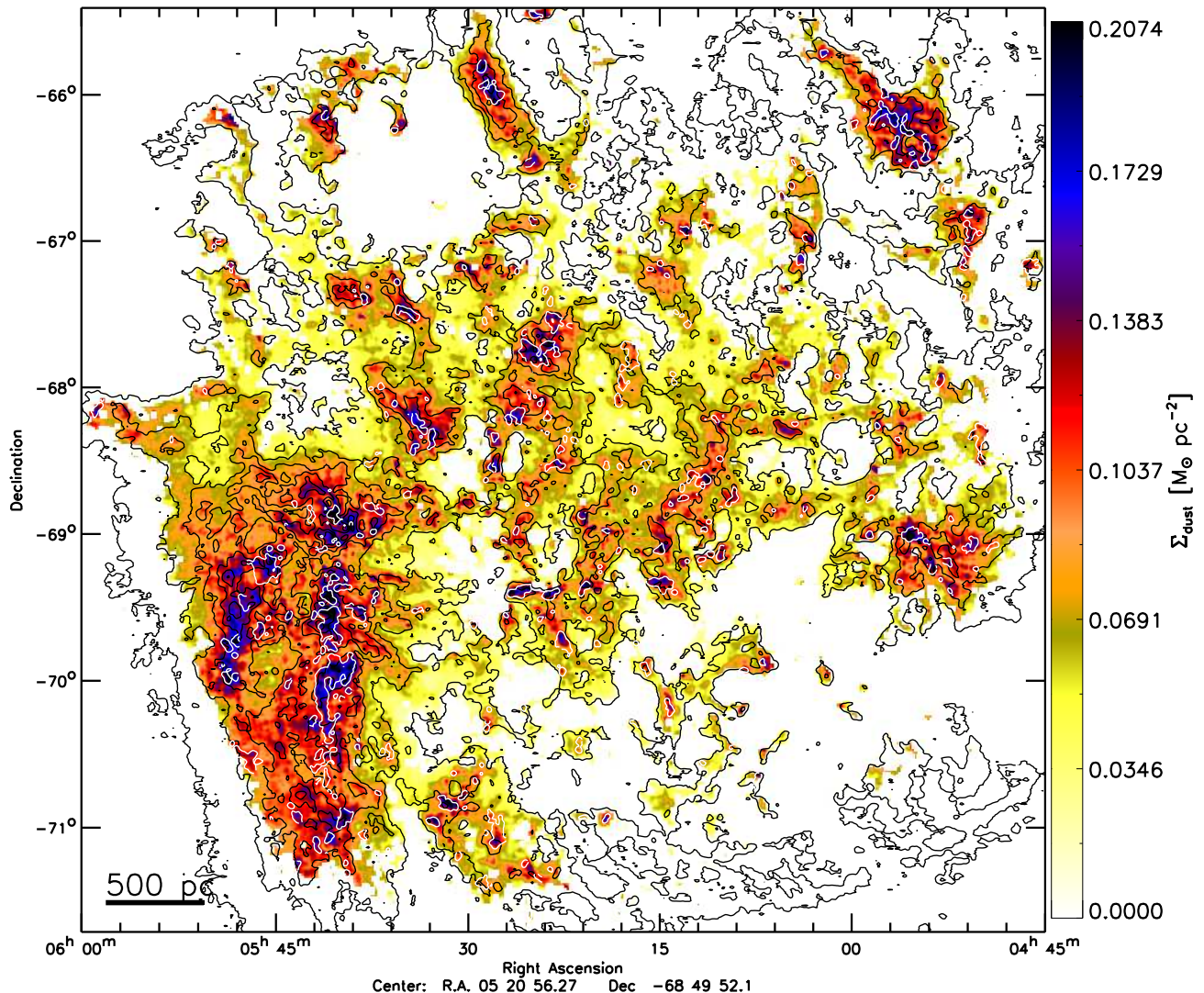
FIG. 1.— Map of the dust surface density in the LMC from Paper I at 1' (15 pc) resolution. The black contours show the H I surface density (Kim et al. 2003), with levels 10\text{--}60 M_{\odot} \text{pc}^{-2} in steps of 10 M_{\odot} \text{pc}^{-2} . The white contours show the CO integrated intensity (Wong et al. 2011), with level 1.2 \text{ K km s}^{-1}
