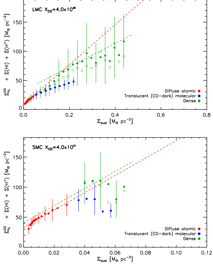
FIG. 15.— Pixel-to-pixel correlation (binned) between dust and total gas (HI, H 2 , H + ) surface densities in the LMC (top) and SMC (bottom), as in Figures 5 and 6, but with the dust surface density obtained by fitting the Herschel/HERITAGE photometry after convolving the FIR maps to the limiting resolution of 1' (LMC) and 2.6' (SMC). Red, blue, and green points correspond to the diffuse atomic, translucent, and dense (CO detected) phases respectively. The filled and empty circles show the binned mean and median. We assume our X_{\text{CO}}^{\text{max}} values, which are found to be 4 \times 10^{20} \text{ cm}^{-2} \text{ K}^{-1} \text{ km}^{-1} \text{ s} in the LMC and 4 \times 10^{21} \text{ cm}^{-2} \text{ K}^{-1} \text{ km}^{-1} \text{ s} in the SMC when the FIR maps are convolved before performing the dust surface density derivation from SED fitting.
