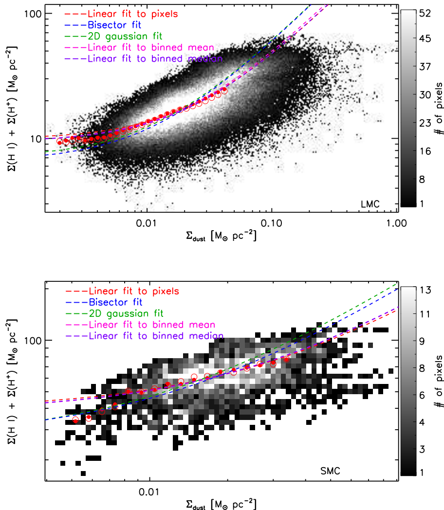
FIG. 10.— Pixel-to-pixel correlation between dust and atomic+ionized gas surface densities in the LMC (top) and SMC (bottom). The grey-scale shows the density of points. The filled red circles show the binned mean atomic gas surface density in the diffuse atomic medium, while the empty red circles show the binned median. Over-plotted are different linear fits. Our fiducial method, which consists in performing a \chi^2 minimization of the pixels to a linear function, is shown as a red dashed line. We also performed a bisector fit (blue), a 2D gaussian fit to the \Sigma_{\text{dust}}-\Sigma(\text{H I}) log-log distribution (green), a linear fit to the binned mean (pink), and a linear fit to the binned median (purple). The resulting dust-gas slopes are summarized in Table 3.
