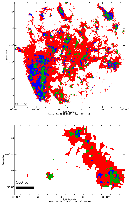
FIG. 7.— Map of the different phases in the LMC (top) and SMC (bottom). The red, blue, and green colors correspond to three different groups of pixels: red points correspond to the diffuse atomic phase and include pixels with \Sigma_{\text{dust}} \leq \Sigma_d^{\text{dif}} and no detectable CO emission (below the 3\sigma_{\text{CO}} sensitivity limit in the SMC, below the sensitivity limit given by the masking algorithm in the LMC). Blue points correspond to the translucent molecular phase, where a significant fraction of the total gas is most likely molecular, but is not traced by CO, and include pixels with \Sigma_{\text{dust}} \geq \Sigma_d^{\text{dif}} and no CO emission. Green points are associated with “dense” pixels with CO emission above the CO sensitivity limit.
