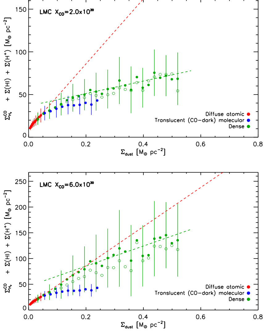
FIG. 5.— Pixel-to-pixel correlation (binned) between dust and total gas (HI, H 2 , H + ) surface densities in the LMC. In the top panel, we assume our fiducial X_{\text{CO}}^{\text{fid}} values for the X factor ( 2 \times 10^{20} \text{ cm}^{-2} \text{ K}^{-1} \text{ km}^{-1} \text{ s} ). In the bottom panel, we assume our X_{\text{CO}}^{\text{max}} values ( 6 \times 10^{20} \text{ cm}^{-2} \text{ K}^{-1} \text{ km}^{-1} \text{ s} ). The red, blue, and green colors correspond to three different groups of pixels: black points correspond to the diffuse atomic phase and include pixels with \Sigma_{\text{dust}} \leq \Sigma_d^{\text{dif}} and no detectable CO emission. Blue points correspond to the translucent phase, where a significant fraction of the total gas is most likely molecular, but is not traced by CO, and include pixels with \Sigma_{\text{dust}} \geq \Sigma_d^{\text{dif}} and no CO emission. Green points are associated with “dense” pixels with CO emission above the sensitivity limit in the integrated intensity, determined by the masking algorithm. Filled circles show the binned mean, while empty circles show the binned median. The best-fit values of the slopes of the dust-total gas relation in the different groups of pixels are indicated in the legend and overlaid as dashed lines.
