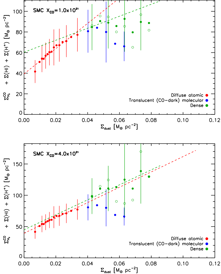
FIG. 6.— Pixel-to-pixel correlation (binned) between dust and total gas (HI, H 2 , H + ) surface densities in SMC. In the top panel, we assume our fiducial X_{\text{CO}}^{\text{fid}} values for the X factor ( 1 \times 10^{21} \text{ cm}^{-2} \text{ K}^{-1} \text{ km}^{-1} \text{ s} ). In the bottom panel, we assume our X_{\text{CO}}^{\text{max}} values ( 4 \times 10^{21} \text{ cm}^{-2} \text{ K}^{-1} \text{ km}^{-1} \text{ s} ). The red, blue, and green colors correspond to three different groups of pixels: black points correspond to the diffuse atomic phase and include pixels with \Sigma_{\text{dust}} \leq \Sigma_d^{\text{dif}} and no detectable CO emission. Blue points correspond to the translucent phase, where a significant fraction of the total gas is most likely molecular, but is not traced by CO, and include pixels with \Sigma_{\text{dust}} \geq \Sigma_d^{\text{dif}} and no CO emission. Green points are associated with “dense” pixels with CO emission above the CO sensitivity limit ( 3\sigma_{\text{CO}} ). Filled circles show the binned mean, empty circles show the binned median. The best-fit values of the slopes of the dust-total gas relation in the different groups of pixels are indicated in the legend and overlaid as dashed lines.
