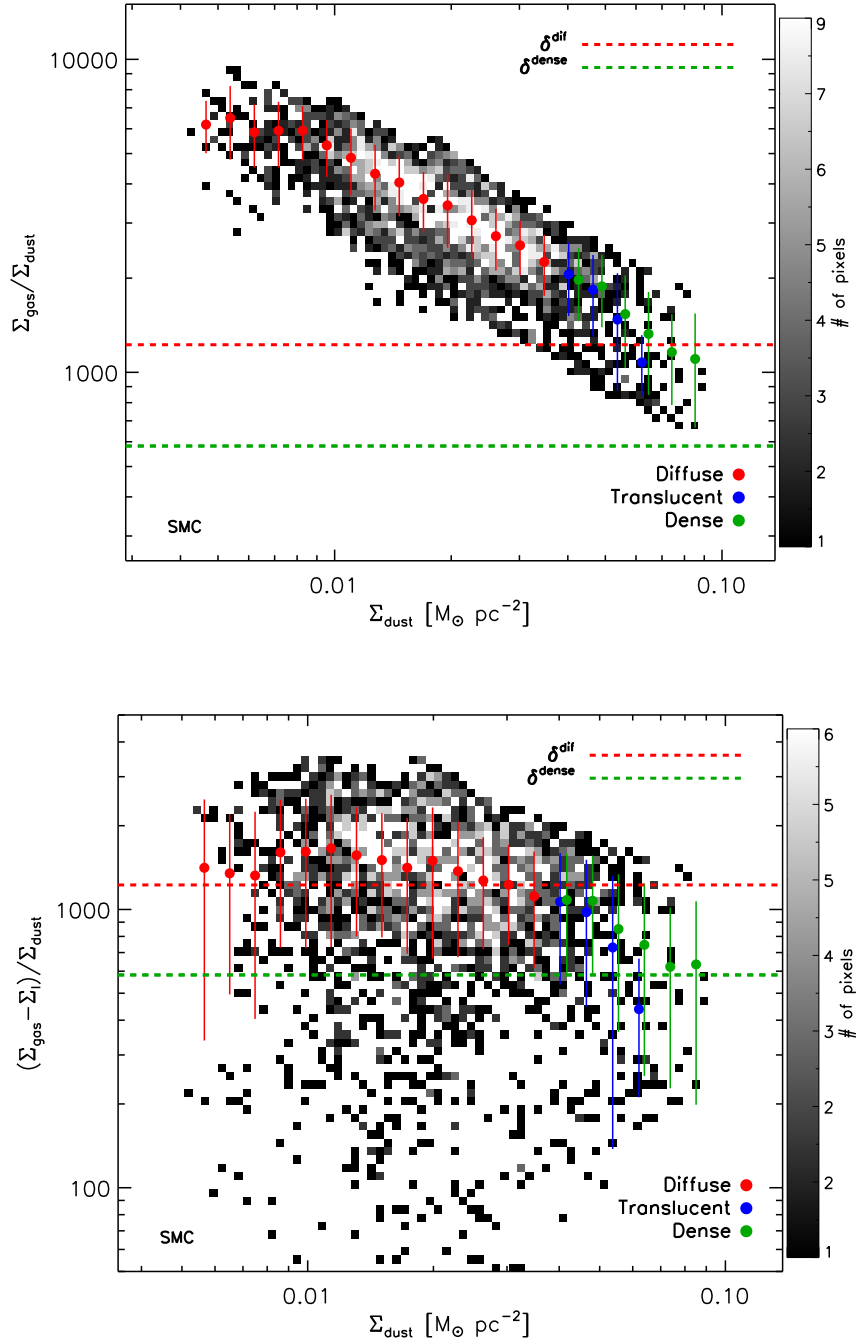
FIG. 9.— Pixel-to-pixel relation between the surface density ratio, which can be interpreted as an apparent gas-to-dust ratio, and the dust surface density for the SMC. Our fiducial X_{\text{CO}} values are assumed. In the top panels, the surface density ratio is computed as \Sigma_{\text{gas}}/\Sigma_{\text{dust}} , while the bottom panels show the surface density ratio after the gas pedestal \Sigma_I is subtracted from the gas, i.e., (\Sigma_{\text{gas}} - \Sigma_I)/\Sigma_{\text{dust}} . Subtracting the gas pedestal is roughly equivalent to computing the surface density ratio in the volume where FIR emission is detected. The contours indicate the distribution of GDR and \Sigma_{\text{dust}} measurements for individual pixels, while the filled circles show the binned mean in each \Sigma_{\text{dust}} bin. The red, blue, and green points correspond to the diffuse, translucent and dense phases. For comparison, the red and green dashed lines correspond to the dust-gas slope values \text{GDR}^{\text{dif}} and \delta_{\text{max}}^{\text{dense}} - \delta_{\text{min}}^{\text{dense}} .
