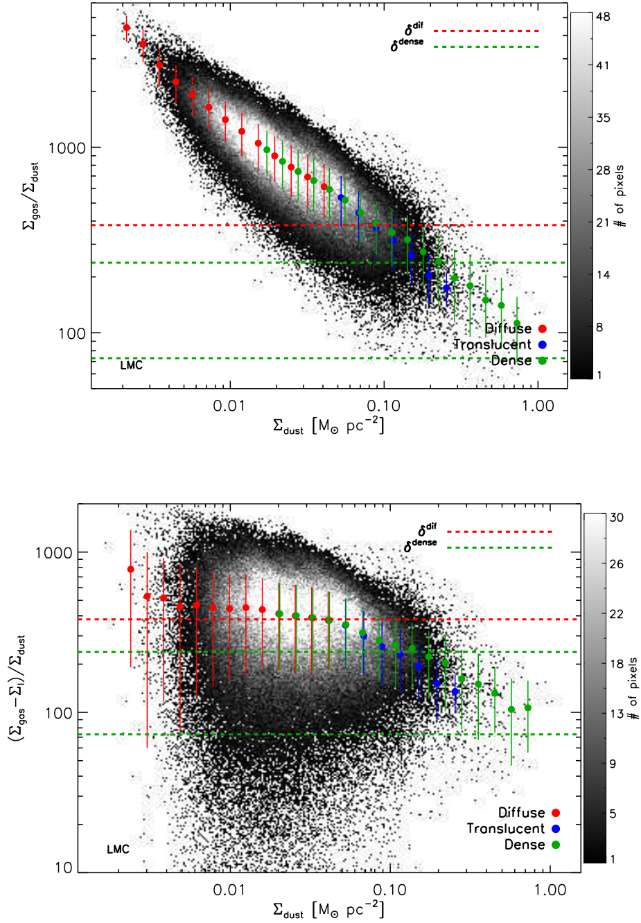
FIG. 8.— Pixel-to-pixel relation between the surface density ratio, which can be interpreted as an apparent gas-to-dust ratio, and the dust surface density in the LMC. Our fiducial X_{\text{CO}} values are assumed. In the top panels, the surface density ratio is computed as \Sigma_{\text{gas}}/\Sigma_{\text{dust}} , while the bottom panels show the surface density ratio after the gas pedestal \Sigma_I is subtracted from the gas, i.e., (\Sigma_{\text{gas}} - \Sigma_I)/\Sigma_{\text{dust}} . Subtracting the gas pedestal is roughly equivalent to computing the surface density ratio in the volume where FIR emission is detected. The contours indicate the distribution of GDR and \Sigma_{\text{dust}} measurements for individual pixels, while the filled circles show the binned mean in each \Sigma_{\text{dust}} bin. The red, blue, and green points correspond to the diffuse, translucent and dense phases. For comparison, the red and green dashed lines correspond to the dust-gas slope values \text{GDR}^{\text{dif}} and \delta_{\text{max}}^{\text{dense}} - \delta_{\text{min}}^{\text{dense}} .
