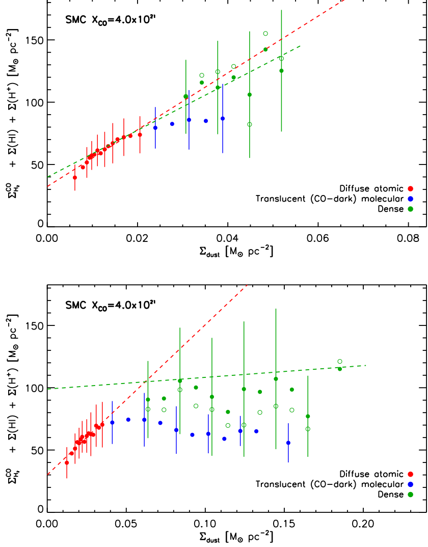
FIG. 13.— Pixel-to-pixel correlation (binned) between dust and total gas (HI, H 2 , H + ) surface densities in the SMC, with the dust surface densities derived from FIR SED fits to the SMBB model (top) and TTMBB model (bottom). The red, blue, and green points and lines correspond to the diffuse, translucent (CO-dark), and dense phases respectively. Filled circles show the binned mean, while empty circles show the binned median. We assume our fiducial X_{\text{CO}} values.
