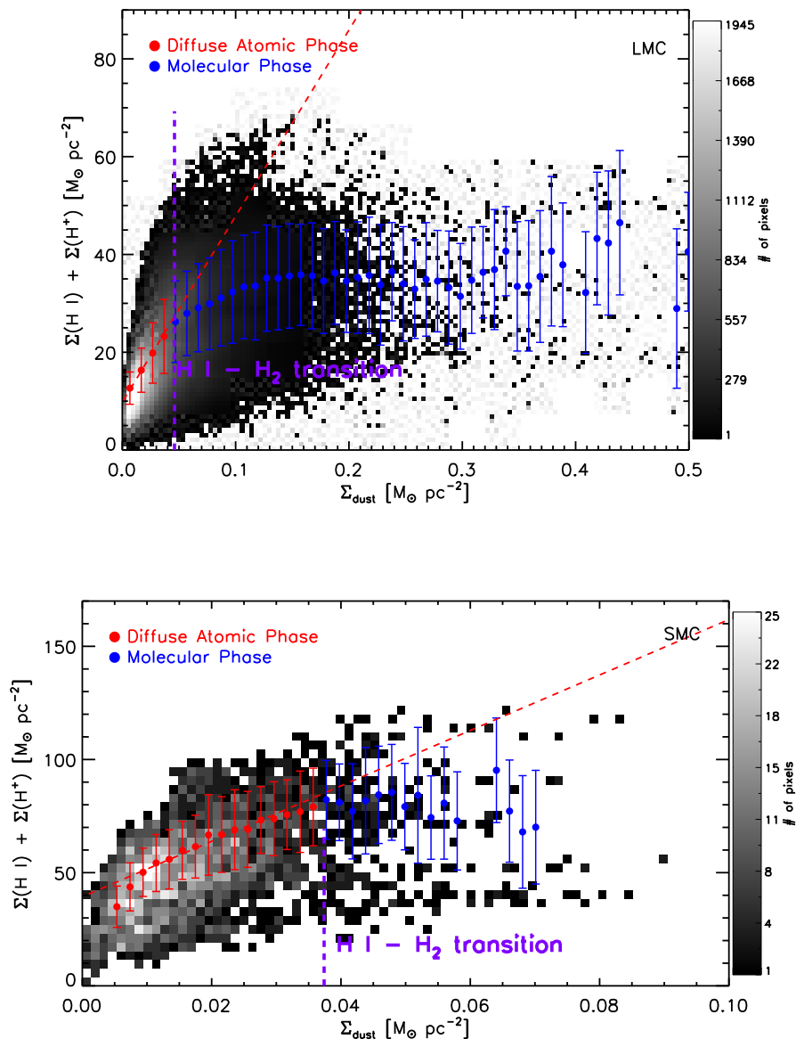
FIG. 3.— Pixel-to-pixel correlation between dust and atomic+ionized gas surface densities in the LMC (top) and SMC (bottom). The grey-scale shows the density of points. The circles show the binned mean. The red and blue colors correspond to the atomic and molecular phases, respectively (see text). The purple dashed line notes the transition point between atomic and molecular. The red dashed line corresponds to a linear fit to the dust-gas slope in the atomic phase, with derived slope of \delta^{\text{dif}} (reported in Table 1). See text and Table 1 for details.
