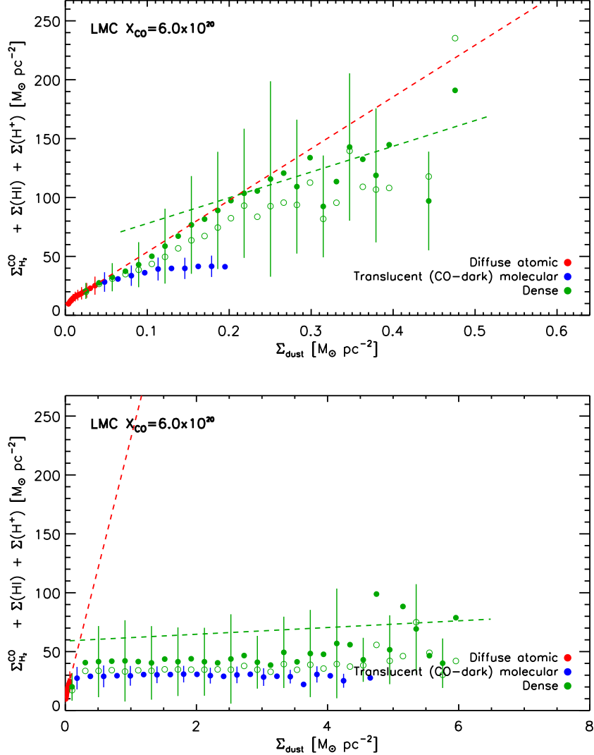
FIG. 12.— Pixel-to-pixel correlation (binned) between dust and total gas (HI, H 2 , H + ) surface densities in the LMC, with the dust surface densities derived from FIR SED fits to the SMBB model (top) and TTMBB model (bottom). The red, blue, and green points and lines correspond to the diffuse, translucent (CO-dark), and dense phases respectively. Filled circles show the binned mean, while empty circles show the binned median. We assume our fiducial X_{\text{CO}} values.
