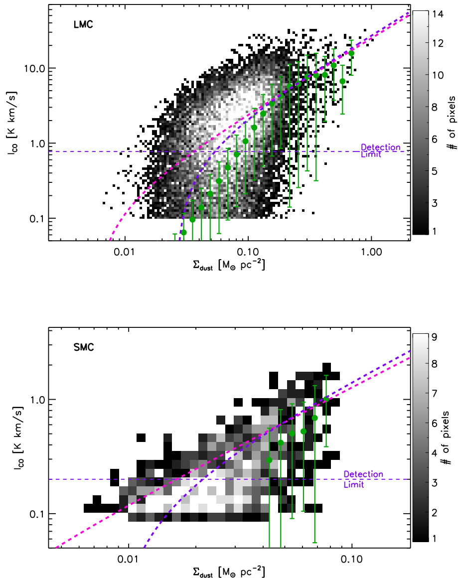
FIG. 4.— Pixel-to-pixel correlation between dust and CO emission in the LMC (top) and SMC (bottom). The grey-scale shows the density of pixels, while the green circles correspond to the binned mean. The sensitivity limit, which corresponds to the 3\sigma_{\text{CO}} noise level in the SMC, and to the detection limit of the masking algorithm in the LMC, is indicated by the horizontal dashed purple line. The slope of the dust-CO relation, \delta^{CO} , is shown as pink (linear fit) and purple (bisector fit) dashed lines.
