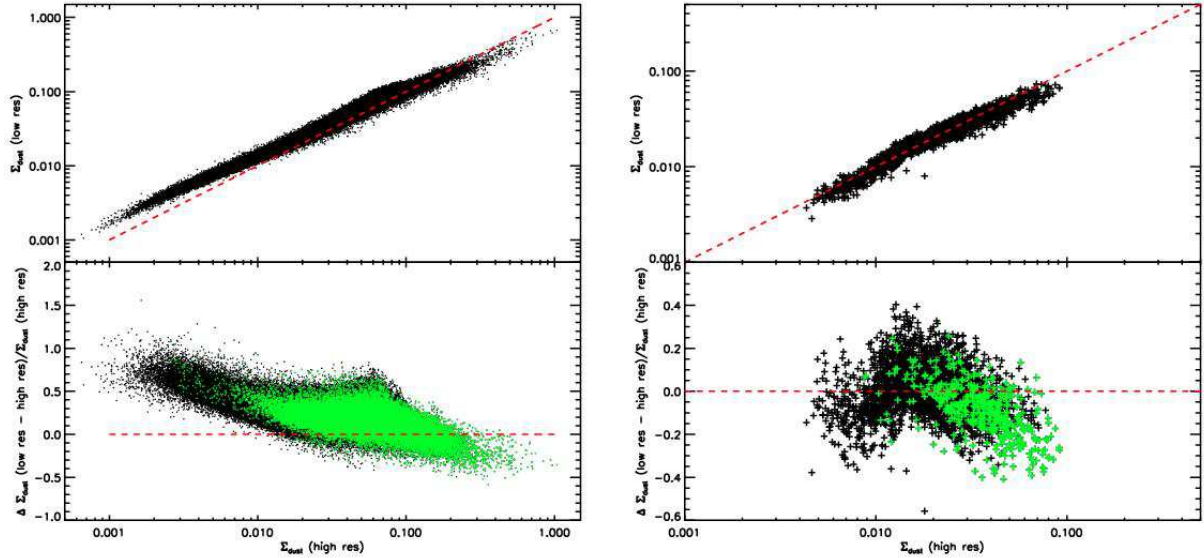
FIG. 14.— Comparison of the “low res” (convolution from Herschel native resolution to limiting resolution applied to the FIR images before SED fitting) and “high res” (convolution applied to the dust surface density maps after SED fitting) dust surface density maps obtained with the BEMBB model, in the LMC (left) and SMC (right). The top panels show the pixel-pixel comparison, while the bottom panels show the fractional difference between the two types of maps. The dashed lines indicate a 1:1 relation. In the bottom panels, black points correspond to pixels with no CO detections while CO is detected in the green points.
