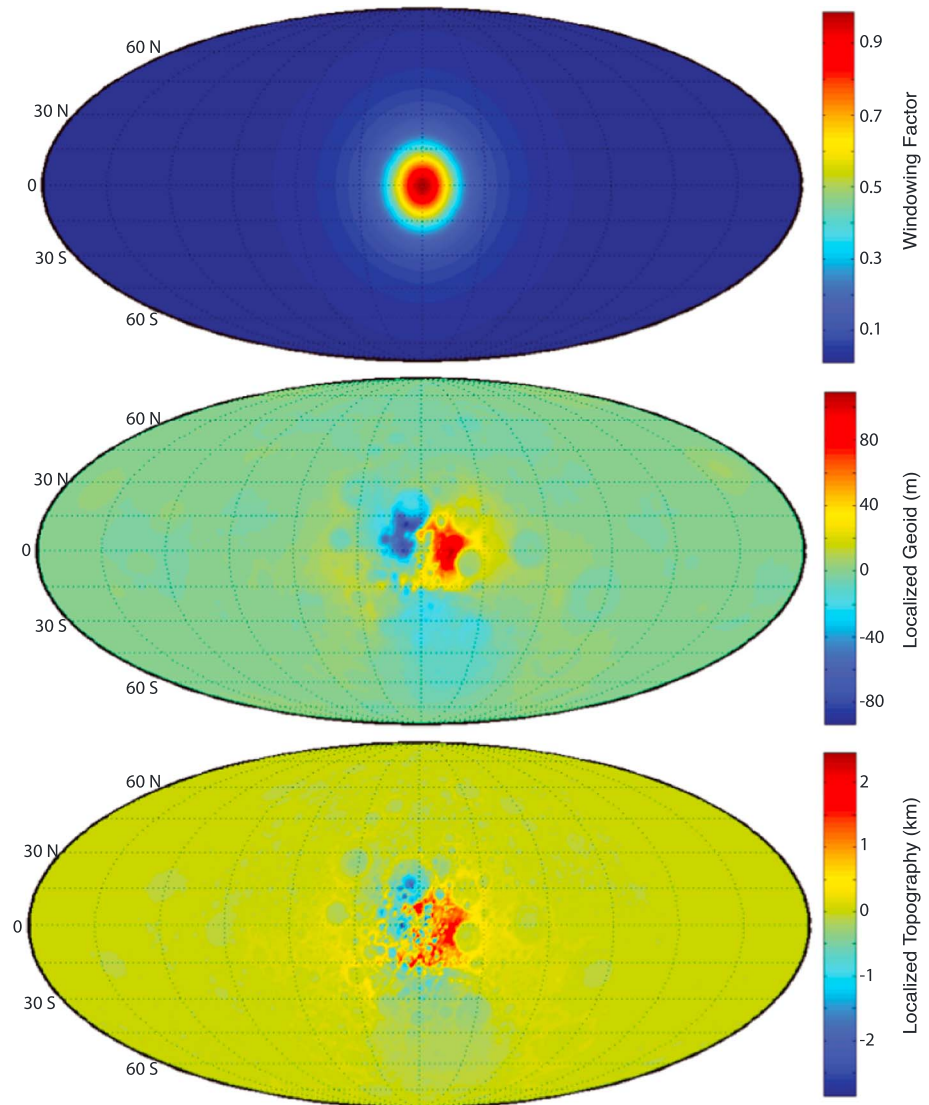
Figure 2. Example of localization of our data. This particular Slepian window (top) was constructed to concentrate optimally its power within a spherical cap of radius 750 km while possessing a spherical harmonic bandwidth of 15. The window was applied to the geoid (middle) and topography (bottom). The maps of localized geoid and topography were then converted back to spherical harmonic coefficients, which were used to calculate the GTR from equation (4). The maps are Mollweide projections centered on the farside.
