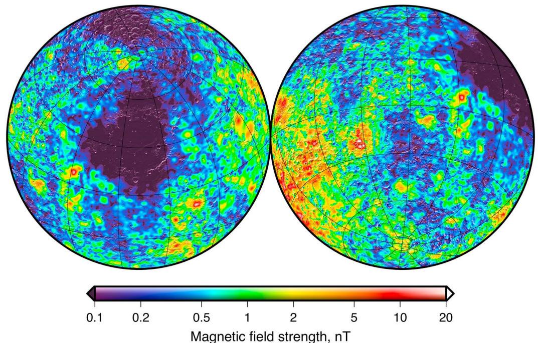
Figure 11. Total magnetic field strength of the Moon at 30 km altitude centered over the (left) Imbrium and (right) Orienteale basins. The field strengths of Tsunakawa et al. (2015) are plotted using a logarithmic color scale, and the maps are presented in Lambert azimuthal equal-area projections overlain by a shaded relief map derived from the Lunar Orbiter Laser Altimeter (Smith et al., 2010). Grid lines are spaced every 30° in latitude and longitude.
