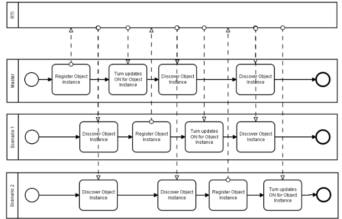
Fig. 5. Object Instance Registration
