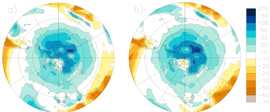
Figure 15. Projected relative change (1980–2000 vs. 2080–2100) of annual precipitation (in %). (a) Uncorrected set of simulations: ([R21-R20]/R20) ; (b) corrected set of simulations: ([C21-C20]/C20) .
