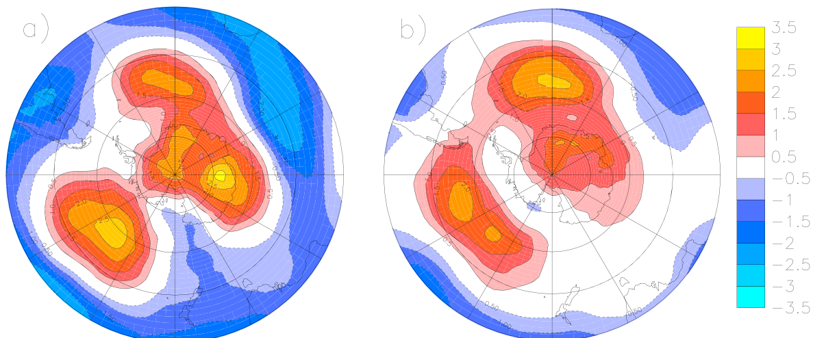
Figure 5. 1980–2000 July air temperature error at 500 hPa with respect to ERA-INT (°C). (a) R20 and (b) C20.
