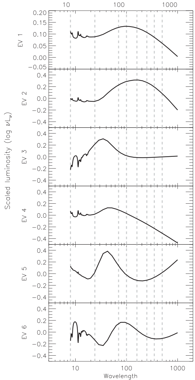
Figure 14. The six main eigenvectors. They, respectively, contain 98.8, 0.53, 0.42, 0.17, 0.06 and 0.02 per cent of the total variance. The 8, 24, 70, 100, 160, 250, 350 and 500\mu\text{m} wavelengths are overlaid as references but the full SED models (sampled with 117 elements) have been used for the decomposition.
