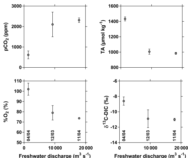
Figure 5. Variation as a function of freshwater discharge ( \text{m}^3 \text{s}^{-1} ) of the partial pressure of CO 2 ( \text{pCO}_2 , ppm), oxygen saturation level ( \% \text{O}_2 , %), total alkalinity (TA, \mu\text{mol kg}^{-1} ), and stable isotope composition of dissolved inorganic carbon ( \delta^{13}\text{C-DIC} , ‰) in the freshwaters (salinity 0) of the three branches of the Mekong delta (Mý Tho, Hàm Luông, and Cồ Chiên) in December 2003, April 2004, and October 2004. Sampling dates (mm/yy) are indicated in the bottom panels.
