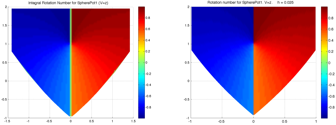
Figure 3: Classical and quantum rotation numbers for an axisymmetric Schrödinger operator on the sphere S^2 . The classical rotation number (left figure) was computed by numerical evaluation of the exact elliptic integral, which is singular on the vertical line I = 0 . The quantum rotation number (right figure) was computed using Formula (49) for I \geq 0 from a numerical diagonalization of the Schrödinger operator; computation for I \leq 0 gives exactly opposite numbers
