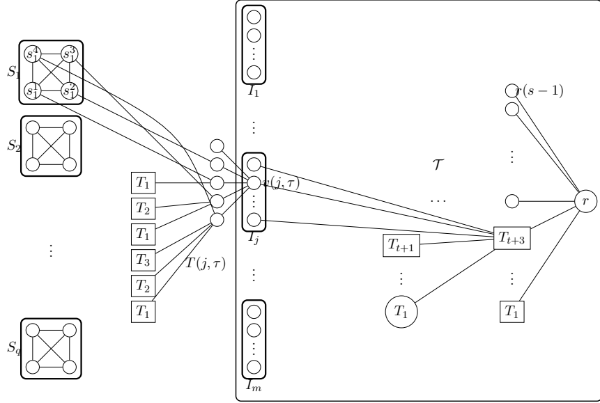
Figure 3: A sample of the construction of graph G . The edges incident to the rectangular boxes containing T_i 's are only incident to the root of the tree. For the sake of readability, only one T(j, \tau) is represented. Here, v(j, \tau) represents an assignment of group X_1 mapped to the permutation \sigma = (12) .
