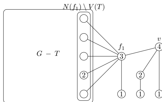
Figure 2: A simple instantiation of Lemma 7 with s = 4 , p = 1 , and a_1 = 2 .
