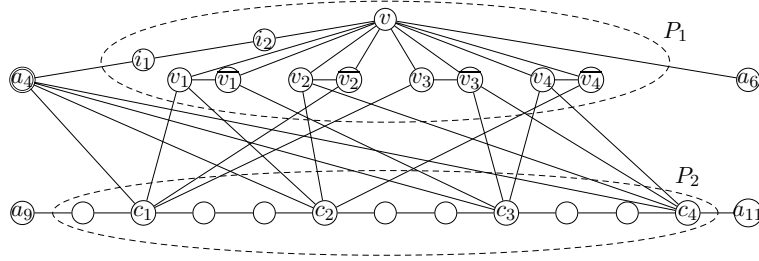
Figure 4: P_1 and P_2 for the instance \{x_1 \vee \neg x_2 \vee x_3\}, \{x_1 \vee x_2 \vee \neg x_4\}, \{\neg x_1 \vee x_3 \vee x_4\}, \{x_2 \vee \neg x_3 \vee x_4\} .
