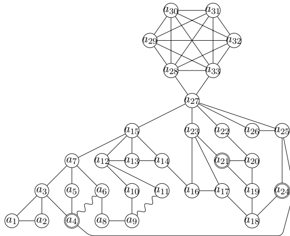
Figure 6: The constant gadget. The doubly circled vertices are adjacent to all the c_j 's ( j \in [m] ).
