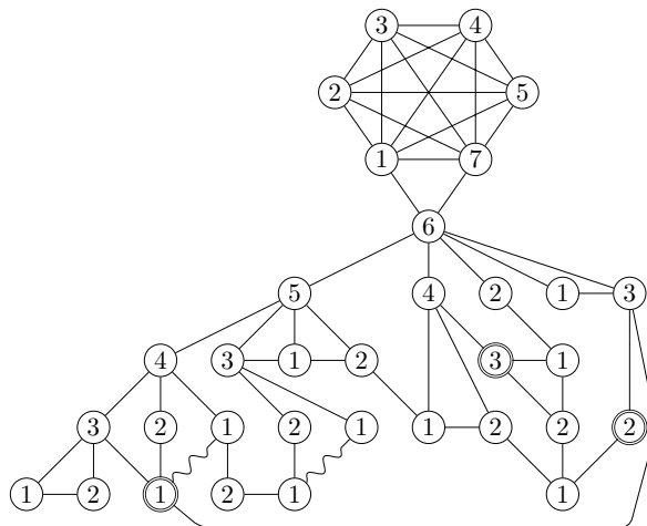
Figure 7: A connected Grundy coloring of the constant gadget achieving color 7. The order is given by the sequence (a_i)_{1 \leq i \leq 33} .
