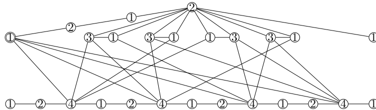
Figure 5: A connected Grundy coloring such that all the c_j 's are colored with color at least 4.
