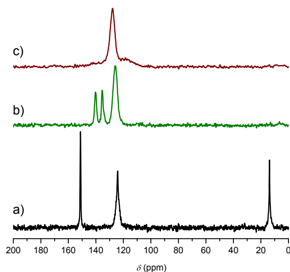
Figure 2. ^1\text{H} decoupled ^{13}\text{C} MAS NMR spectra of (a) ZIF-8_ \text{CH}_3 , (b) ZIF-8_ \text{Cl} and (c) ZIF-8_ \text{Br} .
