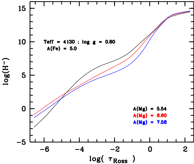
Fig. 1. Number density of H^- vs. optical depth \log \tau_{\text{Ross}} for three different abundances of Mg. The blue line ( A(\text{Mg}) = 7.58 ) corresponds to the solar abundance of Mg, the red line to the Mg abundance in Pisces II 10694, and the black line ( A(\text{Mg}) = 5.54 ) to the Mg abundance expected for a normal metal-poor star with [\text{Fe}/\text{H}] = -2.6 . The molecular bands and the metallic lines are mainly formed between \log \tau_{\text{Ross}} = -2 and -1 , a region where the number density of H^- is strongly affected by the Mg abundance.
