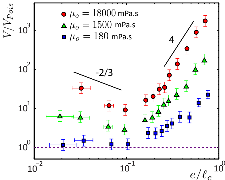
FIGURE 4. Dimensionless velocity \tilde{V} = V/V_{Poiss} as a function of the rescaled gap thickness e/\ell_c , with \ell_c the capillary length. The purple dashed line corresponds to the Poiseuille regime characterized by \tilde{V} = 1 . For most of the experimental measurements, the rescaled velocity \tilde{V} is larger than unity, which enhances the lubricating role of the films of water between the drop and the walls.
