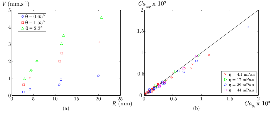
FIGURE 3. (a) Sliding velocity V of drops of silicone oil of viscosity \eta = 4.1 mPa.s bridging the two parallel walls of a Hele-Shaw cell of thickness h = 1100 \mu\text{m} . V increases with the radius R of the drops, and with the apparent gravity, i.e. with the tilt angle \theta of the cell. (b) Measured sliding velocity of drops in a Hele-Shaw cell, expressed in terms of the capillary number Ca_{exp} = \eta V/\gamma as a function of the prediction Ca_{th} of equation 2.15 with \beta = 3.6 . The viscosity \eta of the oils ranges from 4.1 to 44 mPa.s, the drop volume \Omega is between 14 and 1500 \mu\text{L} , the cell thickness h is between 150 and 1100 \mu\text{m} and the tilt angle \theta ranges from 1.4^\circ to 7^\circ . Equation 2.15 is a good prediction of the measured capillary number Ca_{exp} .
