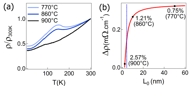
FIG. 4. (Color online) (a) Temperature dependent resistivity curves measured on 770^\circ\text{C} (blue curve), 860^\circ\text{C} (dark blue curve), and 900^\circ\text{C} (black curve) grown 1T - \text{TiSe}_2 crystals. The curves are normalized to the resistivity measured at room temperature. (b) Evolution of the intensity of the resistivity peak as a function of the CDW domains size. The dashed blue curve indicates the typical value of the effective Bohr diameter of excitons in 1T - \text{TiSe}_2 .
