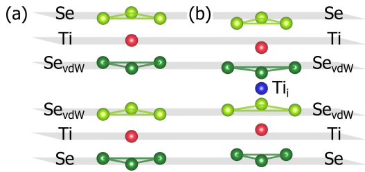
FIG. 3. (Color online) Structural models of 1T - \text{TiSe}_2 as obtained by DFT. Two \text{TiSe}_6 octahedra separated by one vdW gap are considered (a) Pristine 1T - \text{TiSe}_2 (b) Ti-doped 1T - \text{TiSe}_2 . The amplitude of displacements induced by Ti intercalation ( \text{Ti}_i ) have been enhanced.
