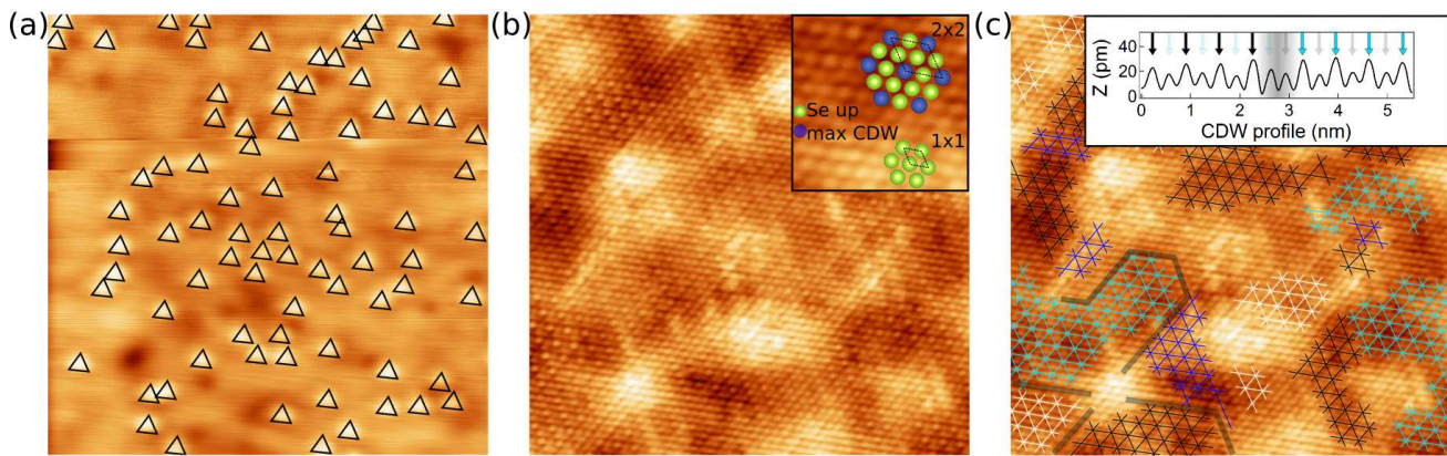
FIG. 1. (Color online) (a) 17 \times 17 \text{ nm}^2 constant current STM images of the 900^\circ\text{C} -grown 1T\text{-TiSe}_2 crystal showing the intercalated-Ti defects (black triangles), V_{\text{bias}} = -1\text{V} , I = 0.2\text{nA} . (b) Constant current STM image at -0.1\text{V} bias voltage and 0.2\text{ nA} current set point of the same region as (a) showing the CDW charge modulation and its perturbation by the presence of Ti defects. The inset presents an eye guide of the 2 \times 2 and 1 \times 1 charge modulations. Green spheres correspond to Se atoms of the topmost layer (Se up) and the blue ones to the maxima of the 2 \times 2 charge modulation (max CDW). (c) Same STM image as (b) with added meshes highlighting the different CDW domains. Four colors have been used to differentiate between the four possible kinds of modulations that are phase shifted to each other. The gray lines show examples where CDW phase-slips occur. The inset shows a height profile through an atomically abrupt CDW phase-slip.
