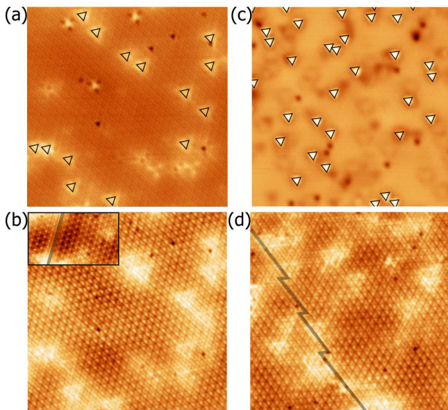
FIG. 2. (Color online) (a) 17 \times 17 \text{ nm}^2 constant current STM image of the 770^\circ\text{C} -grown 1T\text{-TiSe}_2 crystal showing the intercalated-Ti defects (black triangles), V_{\text{bias}} = +1\text{V} , I = 0.2\text{nA} . (b) Constant current STM image at -0.1\text{V} bias voltage and 0.2\text{ nA} current set point of the same region as (a). (c), (d) same as (a), (b) for the 860^\circ\text{C} -grown 1T\text{-TiSe}_2 sample. V_{\text{bias}} = -1\text{V} for (c). The gray lines on (b) and (d) show surface regions where a CDW phase-slip occurs. The inset in (b) is a 7.8 \times 4.5 \text{ nm}^2 constant current STM image showing the presence of a CDW phase-slip on the 770^\circ\text{C} -grown sample.
