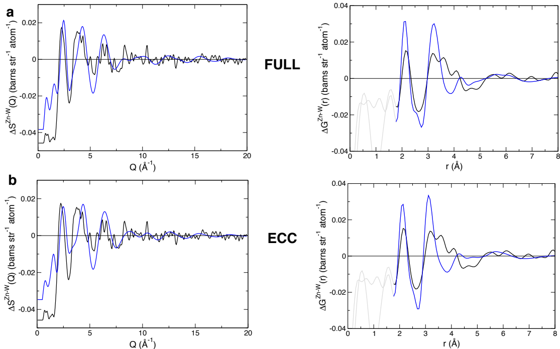
Figure 4: Comparison between the experimental (black) direct difference structure factor \Delta S^{Zn-W}(Q) in Q-space (left hand side) and \Delta G^{Zn-W}(r) in r-space (right hand side) with that obtained with a) the full charges and b) the "ECC" force field for Zn^{2+} .
