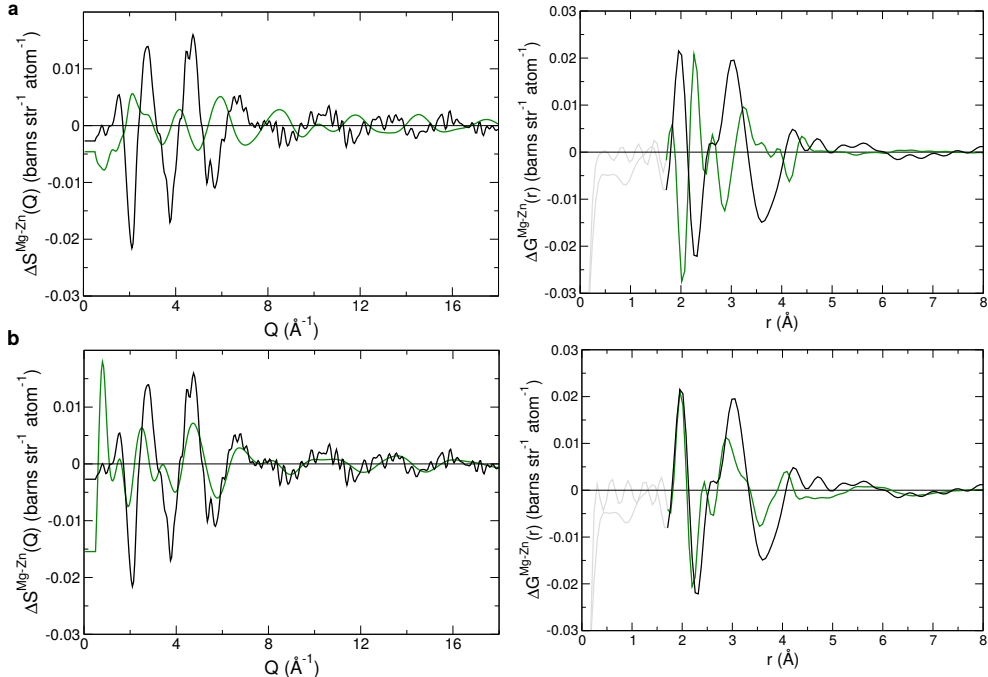
Figure 9: Comparison between the experimental (black) direct difference structure factor \Delta S^{\text{Mg-Zn}}(Q) in Q-space (left hand side) and \Delta G^{\text{Mg-Zn}}(r) in r-space (right hand side) with that obtained with a) the full charges or b) our best ECC force field ("ECC small" for \text{Mg}^{2+} and "ECC+ \sigma_{\text{ZnCl}} " for \text{Zn}^{2+} ).
