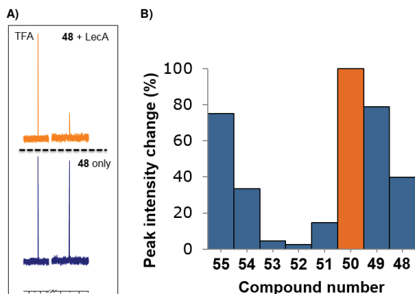
Figure 6. Direct observation of 19 F resonances of monofluorinated galactosides upon binding to LecA. A) 19 F NMR spectrum of compound 48 (blue) and in presence of LecA (orange): Reduction of the signal intensity of the galactoside indicates binding to LecA. Both spectra were normalized to reference trifluoroacetic acid (TFA: -75.6 ppm). B) Percent peak intensity changes of 19 F monofluorinated galactosides 48–55 in presence of LecA (blue) compared to spectra recorded in absence of LecA. Compound 50 was arbitrarily assigned with 100% to indicate binding inferred from chemical shift perturbation (orange) in absence of intensity reduction.
