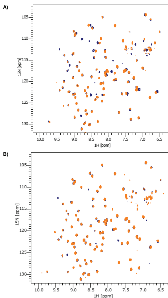
Figure 4. Chemical shift perturbations of backbone resonances of LecA upon binding to galactose derivatives 48 and 52 using ^1\text{H},^{15}\text{N} -TROSY NMR experiments. Spectra of 350\ \mu\text{M} ^{15}\text{N} -labelled LecA in the absence (blue) and presence (orange) of monofluorinated galactoside are shown for A) 0.2\ \text{mM} 48 and B) 1.0\ \text{mM} 52 . Fluorination in C2 ( 48 ) induces multiple chemical shift perturbation and line broadening while fluorine atom at C-4 ( 52 ) abrogates binding to LecA.
