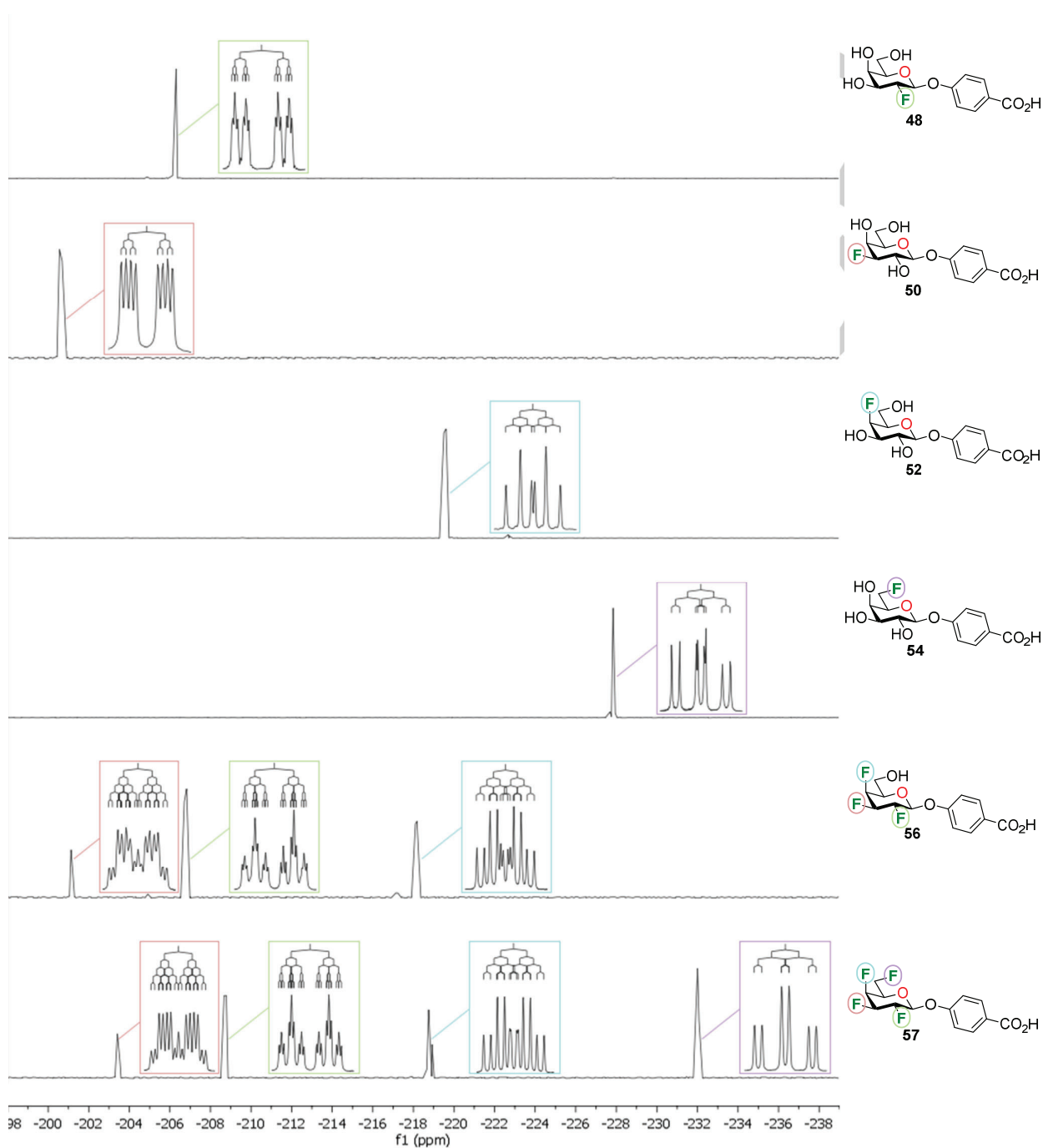
Figure 3. Direct comparison of ^{19}\text{F} resonances of compounds 48, 50, 52, 54, 56, and 57 ( ^{19}\text{F} NMR, 470 MHz). Expansions from the spectrum display coupling constant of each signals.
