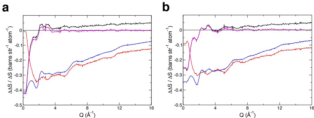
FIG. 2. Experimental first order differences \Delta S(Q) in H 2 O (red) and D 2 O (blue) for a) a 3 m imidazole solution and b) a 3 m imidazolium chloride solution, together with the corresponding second order differences \Delta\Delta S(Q) , before (in black) and after (magenta) a correction to remove the residual Placzek.
