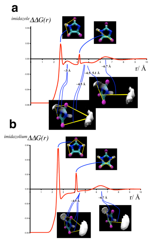
FIG. 5. Second order differences in the r -space \Delta\Delta G(r) as obtained from MD simulations of a) an imidazole solution and b) an imidazolium chloride solution. The origin of each characteristic feature is identified in the corresponding inset, either a molecular correlation (upper insets) or a hydration pattern, as reflected with the density map for H_{ex} around the solute (lower insets).
