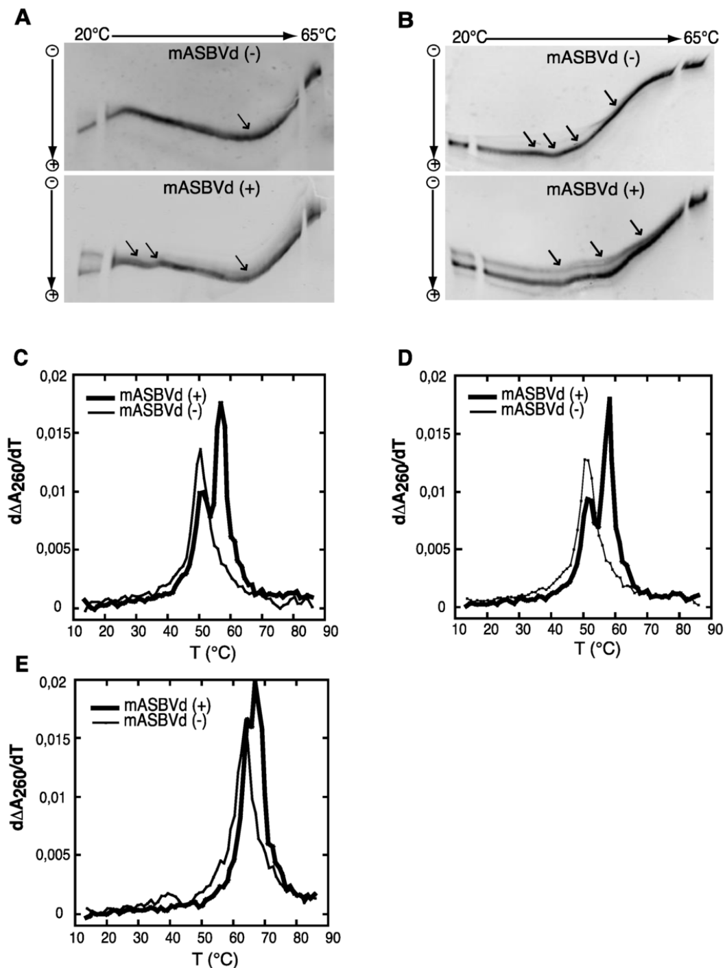
Figure 2. TGGE (Thermal Gradient Gel Electrophoresis) and melting curves of the monomeric forms of ASBVd: mASBVd (+) and mASBVd (−) transcripts. (A) TGGE analysis performed by native gel electrophoresis 8% PAGE in 0.2 TBE Buffer. (B) TGGE analysis performed by native gel electrophoresis 8% PAGE in 0.2 TBE Buffer containing 20 mM magnesium acetate. Migration was monitored between 20 °C and 65 °C. The arrows denote the transition temperatures. Derivative absorbance melting profiles were determined either in 150 mM KCL and 10mM sodium cacodylate (pH 7.2). (C) or with in addition, 100 mM MgCl 2 (D) or 1M NaCl. (E) The first derivative profiles are shown with a thick curve for mASBVd (+) and a thin curve for mASBVd (−). The apparatus fixes the temperature gradient, which is transferred from left to right on the figure; the arrows indicate the transition temperatures that correspond to the conformational changes. From Delan-Forino et al. [70].
