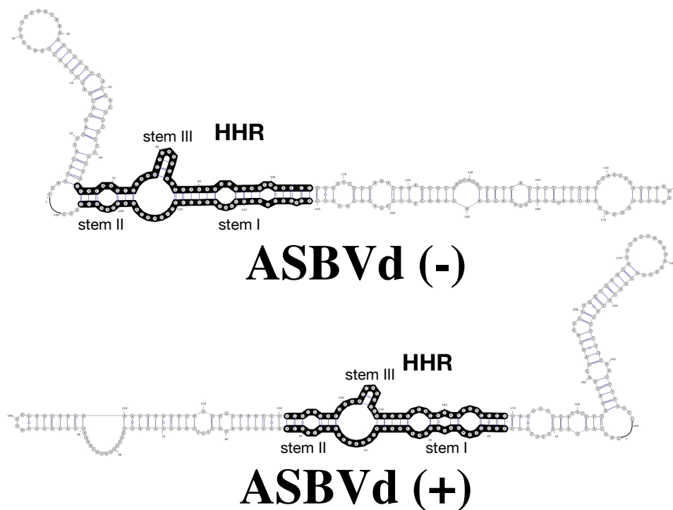
Figure 1. RNA 2D structures of Avocado Sun Blotch Viroid (ASBVd) (–) and ASBVd (+) (top and bottom, respectively). The full length genome of ASBVd can fold into 2D structures that preserve the hammerhead ribozyme (HHR) motif (regions in black) in both the (–) and (+) strands; the HHR motif of ASBVd (–) is more stable, with 3 base-pairs in stem III but only two base-pairs in ASBVd (+).
