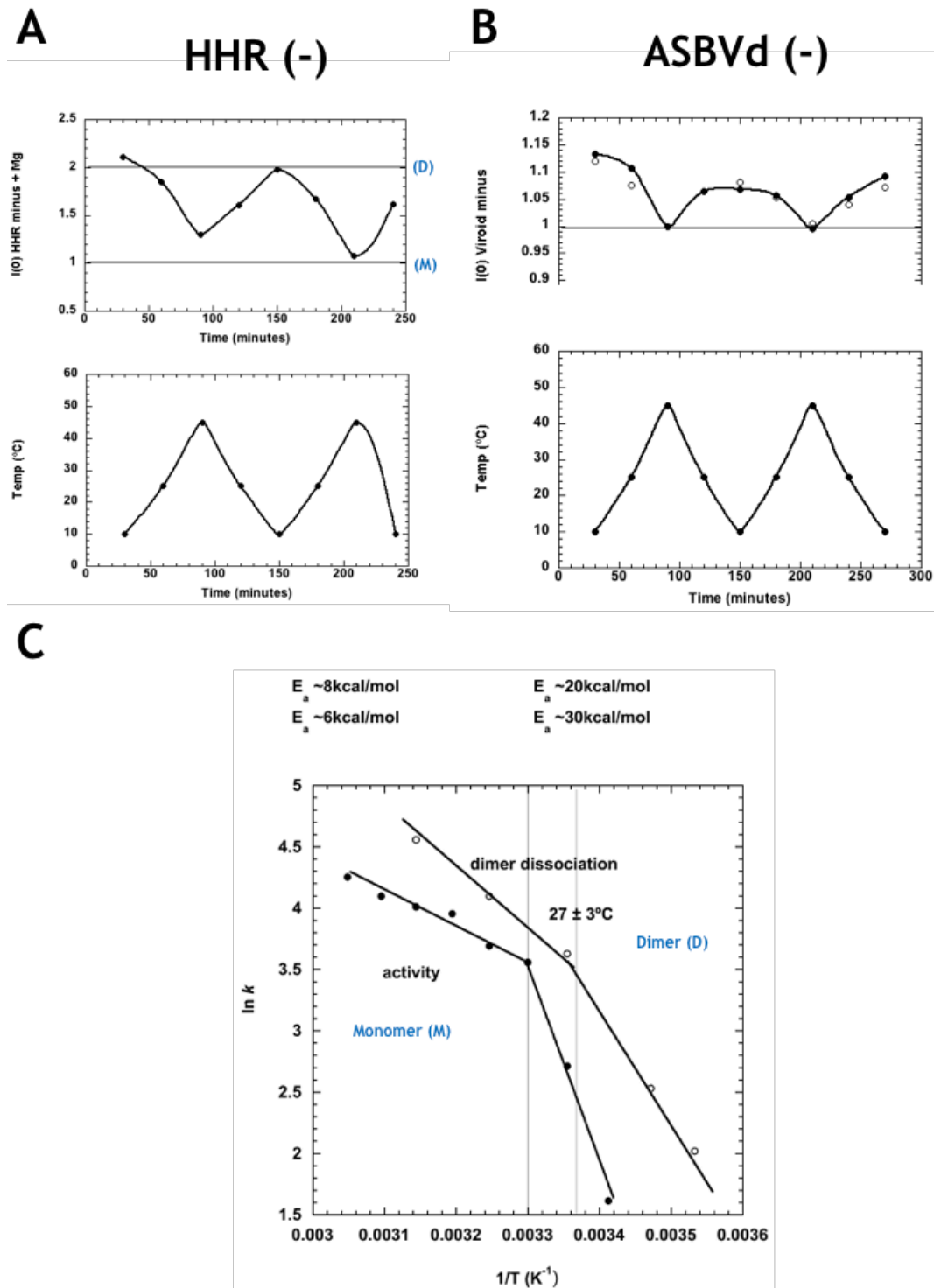
Figure 3. (A) Normalized forward scattered small-angle neutron scattering (SANS) intensity for HHR (–) in the presence of Mg ++ at the corresponding temperature on the plot below. The values at 1.00 and 2.00 correspond to the intensity expected for the monomer (M) and dimer (D), respectively. (B) Normalized forward scattered SANS intensity for ASBVd (–) in presence (filled circles) and absence (open circles) of Mg ++ , at the corresponding temperature on the plot below. The data indicate a small amount of dimer formation at the lower temperature. (C) Arrhenius plots of HHR (–)/Mg rate of dimer dissociation (open circles, calculated from (A)), and the ribozyme’s catalytic activity (filled circles), revealing parallel behaviour. Modified from Leclerc et al. [33].
