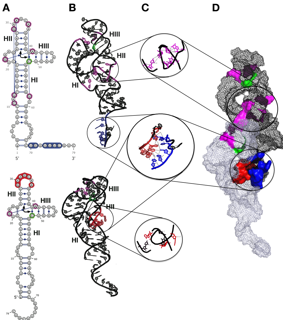
Figure 4. 3D Model of self-association for the hammerhead ribozyme (HHR) from ASBVd(-). (A) 2D structures of the two monomers as they are in the HHR dimer. (B) 3D structures of the two monomers as they are in the HHR dimer. (C) Zoom in on the regions involved in the monomer-monomer interactions and in the 3D contacts within the first monomer (top). (D) 3D structure of the HHR dimer. The long-range intramolecular contacts are indicated in magenta and the cleavage site in green. The paired regions are blue (first monomer) and red (second monomer). Modified from Leclerc et al. [33].
