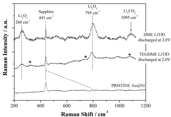
Figure 2. Raman spectra of the Au@Ni electrodes recuperated from Li-O 2 cells after discharge to 2.0 V in TEGDME and DME electrolytes. Broad bands indicated by (*) are possibly due to the LiTfO salt.
