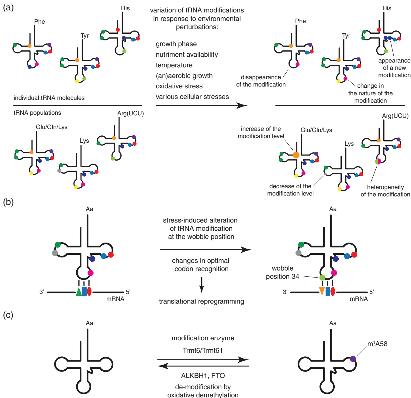
FIG 4 Dynamic changes in tRNA modification levels. (a) Variations of tRNA modifications in response to environmental perturbations. In response to various environmental or cellular factors, such as growth phase, nutriment availability, temperature, aerobic versus anaerobic growth, oxidative stress, or various cellular stresses, the levels and/or the nature of certain modifications can change in tRNAs. Variations occur at the level of individual tRNA molecules (disappearance of a modification, appearance of a new modification, and change in the nature of the modification). These variations collectively impact the level of modifications in tRNA populations, such as particular isoacceptors (e.g., tRNA Lys ) or isodecoders (e.g., tRNA Arg(UCU)} ). In a certain tRNA population, these variations may appear in the form of increased or decreased modification levels, or may introduce modification heterogeneities at certain positions. (b) Stress-induced alteration of tRNA modification at the wobble position can lead to translational reprogramming. Stress-induced alteration of tRNA modification at the wobble position 34 changes the optimal codon recognition of the given tRNA and thereby upregulates the formation of critical stress-response proteins encoded by mRNA transcripts enriched in this particular codon adapted to the altered wobble modification. (c) Variations in tRNA modifications and active demodification processes. The m^1A58 modification, introduced in human by the Trmt6/Trmt61 modification enzyme, can be actively removed by the demodification enzymes ALKBH1 and FTO via an oxidative demethylation process.
