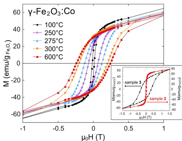
FIG. 2. (Color online) Magnetization vs magnetic field measured at 10 K for \gamma -Fe 2 O 3 :Co NPs (1) embedded in silica (Fe/Si=0.008) after annealing at selected temperatures. In inset, M(H) curves for the \gamma -Fe 2 O 3 /SiO 2 composite (2) after drying at 100 °C and for sample 3. Samples were cooled under zero magnetic field before measurements.
