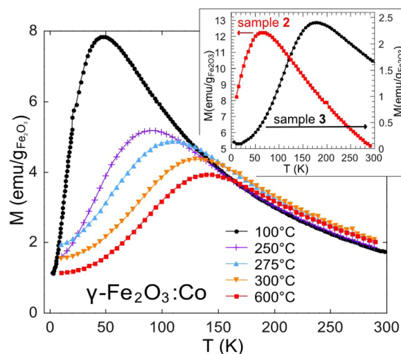
FIG. 1. (Color online) ZFC curves for \gamma -Fe 2 O 3 :Co NPs (1) embedded in silica (Fe/Si = 0.008) annealed at 100, 250, 275, 300, and 600 °C. In inset, ZFC curves for the \gamma -Fe 2 O 3 /SiO 2 composite (2) after drying at 100 °C and for sample 3. All measurements were performed under 25 G magnetic field.
