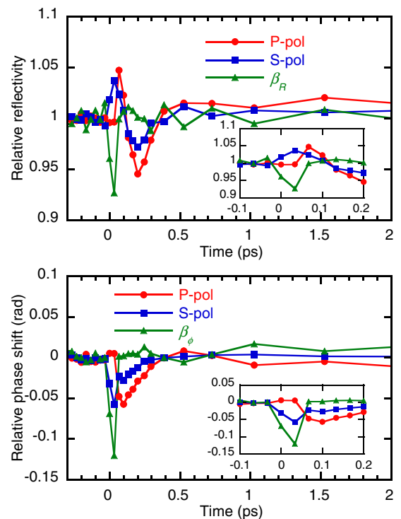
FIG. 4. Time evolution of the reflectivity (top) and phase shift (bottom), relative to an unexcited \text{SiO}_2 sample when a 50- \text{TW cm}^{-2} pump pulse excitation is used. The insets show a zooming for the very short delays.
