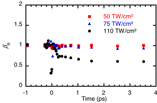
FIG. 3. Time evolution of \beta_R = R_P/R_S^2 for three intensities below (50), around (75), and above (110 \text{TW cm}^{-2} ) the ablation threshold on the \text{SiO}_2 sample. The error bars are approximately the size of the symbols.
