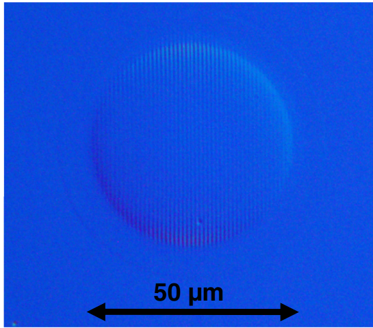
FIG. 5. Nomarsky microscope image of the SiO 2 sample when pump and probe pulses temporally overlap. The center intensity of the pump pulse is 160 TW cm -2 .
