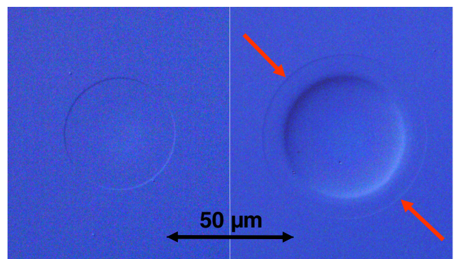
FIG. 2. Nomarsky microscope images of the \text{SiO}_2 sample after irradiation by one laser pulse of the center intensity of 75 \times 10^{12} \text{ W cm}^{-2} (left) and 160 \times 10^{12} \text{ W cm}^{-2} (right). The pronounced feature in the right image is a 200 \pm 10 -nm depth hole, whereas the light feature highlighted by the red arrows is a damage without ablation (no measurable depth).
