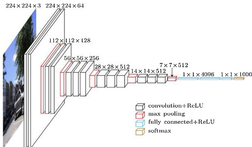
Fig. 1. VGG16 architecture [14].
