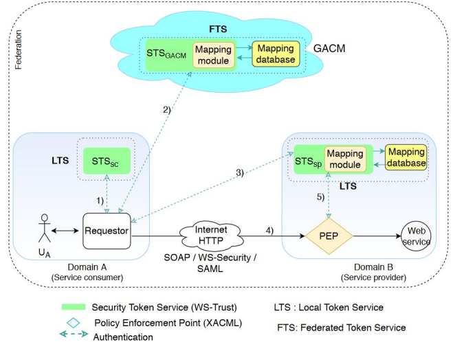
Figure 6: The required software modules and their customizations for the implementation
