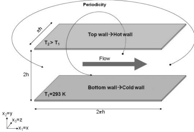
Figure 2 Studied configuration.
