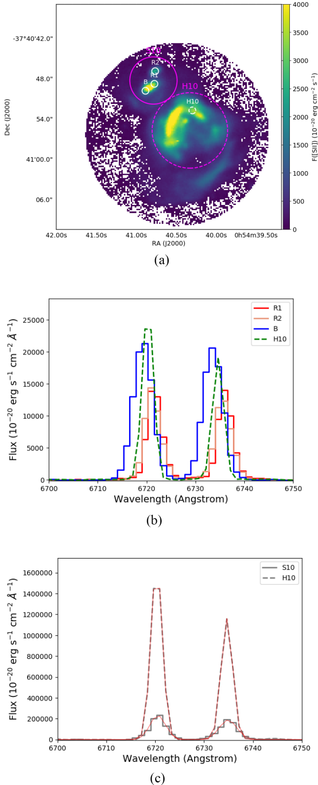
Figure 4. Panel (a): [S II] \lambda 6717 integrated line map. The white circles indicate the regions used to extract the spectra shown in panel (b), while the magenta circles show the regions used to extract integrated spectra for S10 and H10, shown in panel (c). Dashed circles refer to H10, solid circles to S10. Panel (b): continuum-subtracted spectra of the blue- and redshifted lobes and H10 cropped around the [S II] \lambda\lambda 6717, 6731 lines, extracted from the white regions shown in panel (a). Panel (c): same as panel (b) for the magenta regions, red lines are Gaussian fits (see Table 2).
