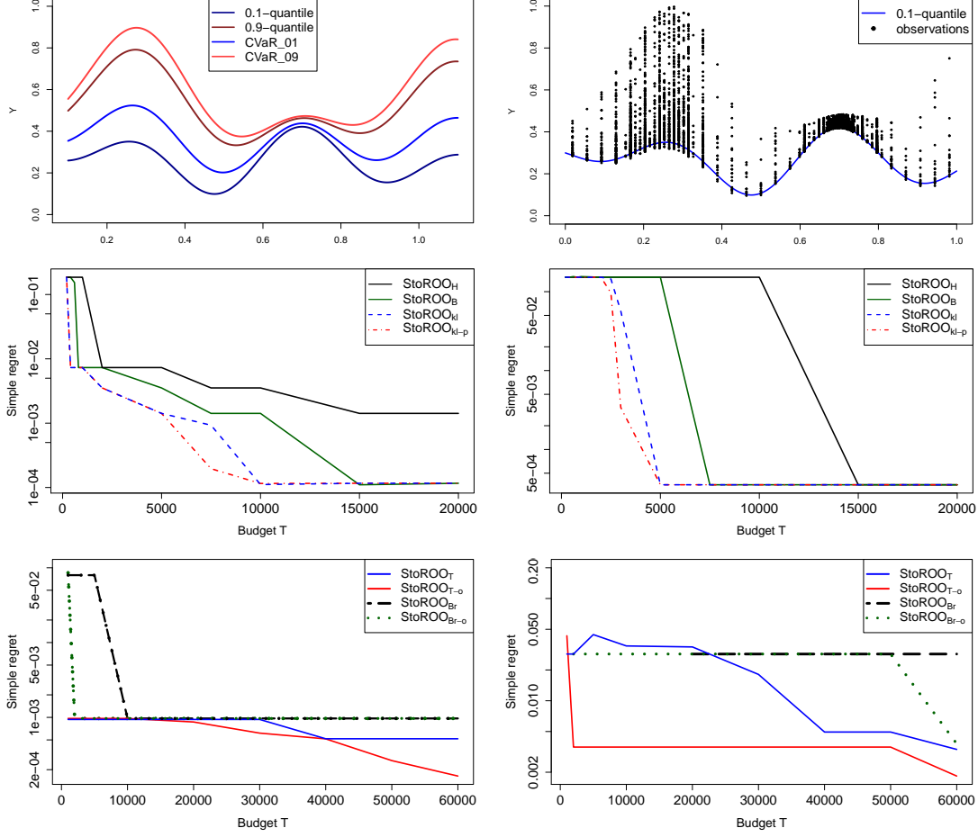
Figure 2: Results for the \Phi_1 test function. Top left: conditional quantiles and CVaR of \Phi_1 . Top right: one run of StoROO kl for the 0.1-quantile with T = 5,000 , \hat{\beta} = 12 and \hat{\gamma} = 1.4 . Middle: evolution of the simple regret for the optimization of the quantile of order 0.1 (left) and 0.9 (right). Bottom: evolution of the simple regret for the optimization of the CVaR of order 0.1 (left) and 0.9 (right).
