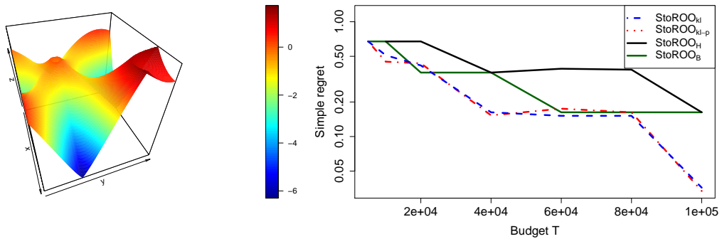
Figure 3: Results for the \Phi_2 test function. Left: Conditional quantile of order 0.1 of \Phi_2 . Right: Simple regret for the optimization of the conditional quantile presented to the left.
