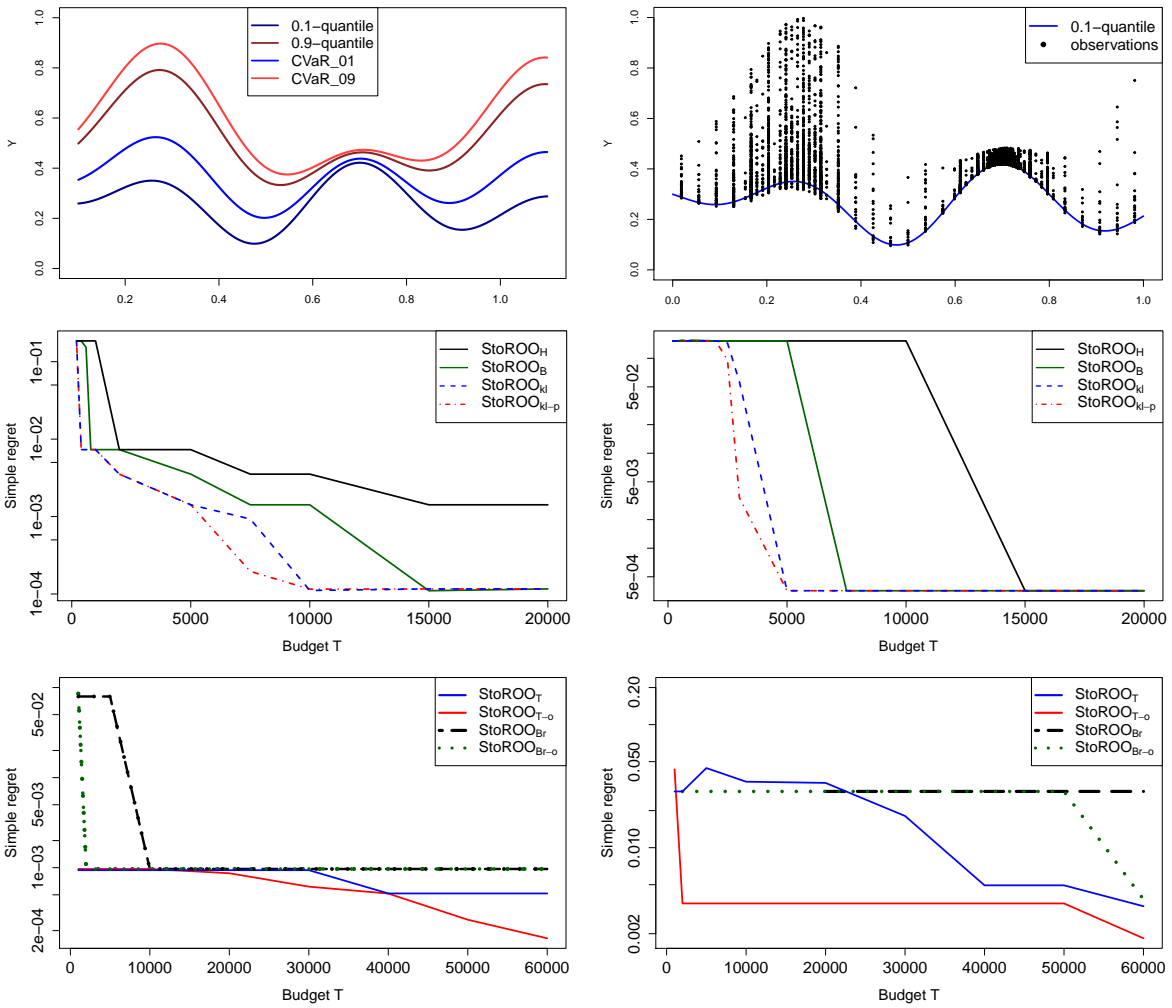
Figure 2: Results for the \Phi_1 test function. Top left: conditional quantiles and CVaR of \Phi_1 . Top right: one run of \text{StoROO}_{kl} for the 0.1-quantile with T = 5,000 , \beta = 12 and \gamma = 1.4 . Middle: evolution of the simple regret for the optimization of the quantile of order 0.1 (left) and 0.9 (right). Bottom: evolution of the simple regret for the optimization of the CVaR of order 0.1 (left) and 0.9 (right).
