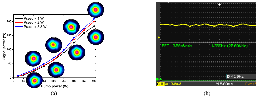
Figure 1: (a) Evolution of the output signal power versus pump power for three different seed power levels ( P_{\text{seed}} = 1\text{ W} / 2\text{ W} / 3.8\text{ W} ) for the 84 \mu\text{m} core fiber ( \Delta n = +8 \times 10^{-5} ) in nanosecond regime. Inset: measured far-field intensity distributions for several signal power levels for P_{\text{seed}} = 1\text{ W} and P_{\text{seed}} = 3.8\text{ W} . (b) Measured time trace (in yellow) and Fourier spectrum (in green) for an extracted signal power of 210 W ( P_{\text{seed}} = 3.8\text{ W} ).
