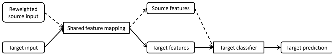
Fig. 4. Illustration of Knowledge Transfer from re-weighted source data to target classifier parameters
