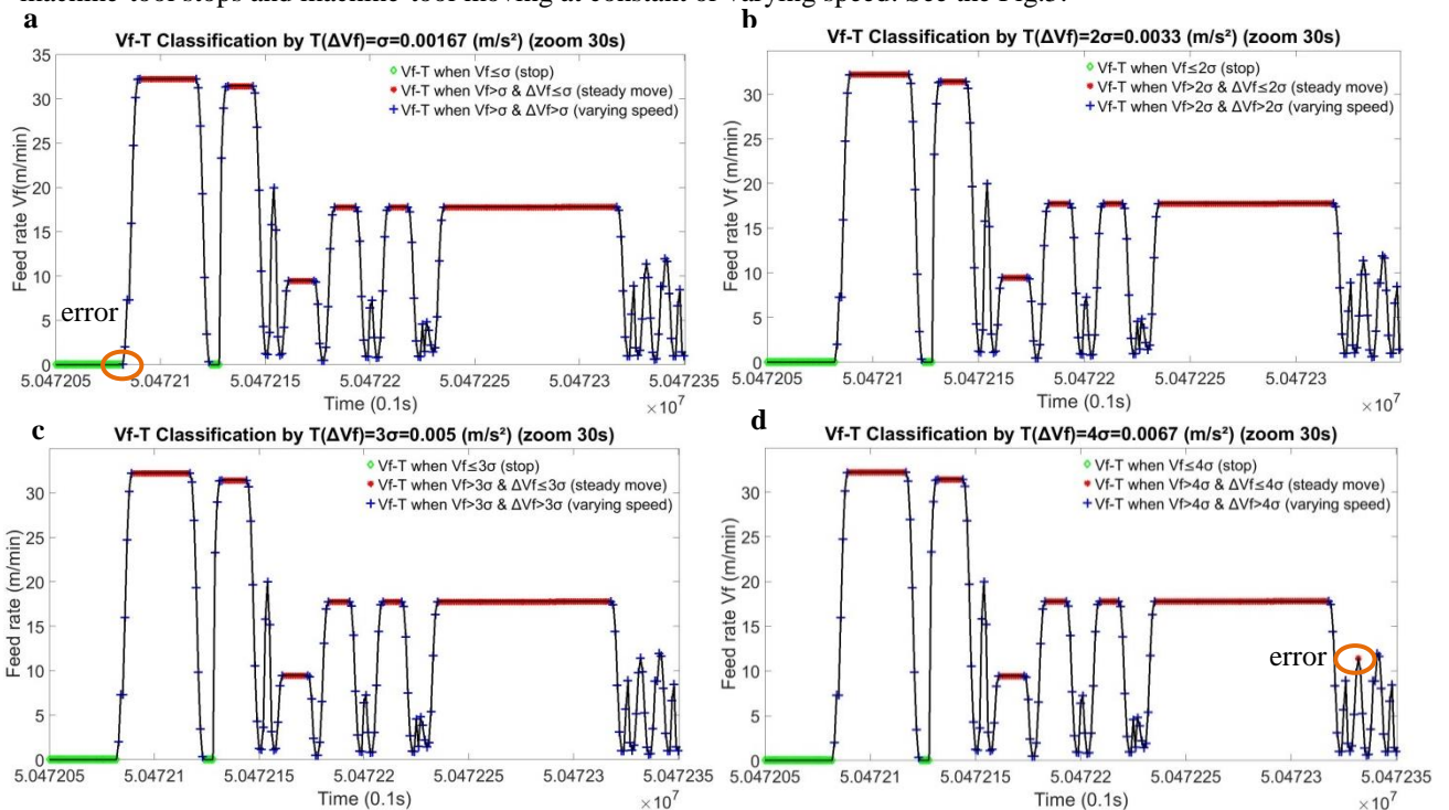
Fig. 5. (a) Vf-T according to 1\sigma classification of \Delta Vf during 30 seconds; (b) Vf-T according to 2\sigma classification of \Delta Vf during 30 seconds; (c) Vf-T according to 3\sigma classification of \Delta Vf during 30 seconds; (d) Vf-T according to 4\sigma classification of \Delta Vf during 30 seconds;
