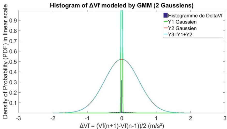
Fig. 4. Density of probability of \Delta V_f for one day modeled by GMM (2 Gaussiens).
