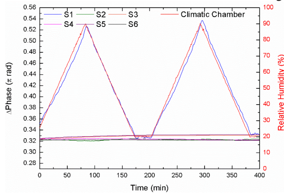
Fig. 9. S1 performance towards relative humidity variations.
