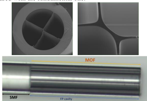
Fig. 2. MOF-4-Bridge cross section (SEM picture) and a resulting FP cavity (microscope picture).
