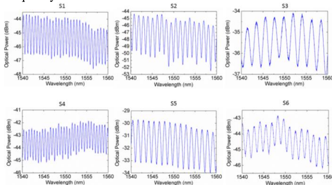
Fig. 3. Sensor's individual optical spectrum.
