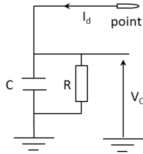
Fig. 3: Mean current measurement device. R represents the input impedance of the voltage probe.
