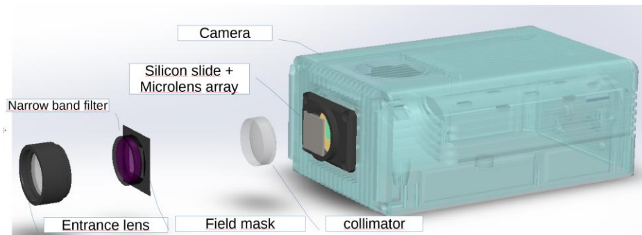
Figure 4. Sketch of optics for the Nanocarb instrument.
