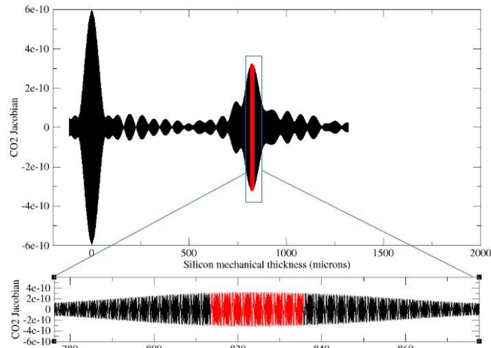
Figure 5. Jacobian of the CO 2 molecule is the sensitivity to a variation of CO 2 concentration of 1ppm. This jacobian is plotted along the width of interferometer. In red, the ideal silicon depth is comprised between 817 \mu m and 835 \mu m.
