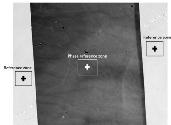
Figure 10. Relative phase variation map obtained with the cross-spectrum method. The phase variations are given with respect to the reference position.
