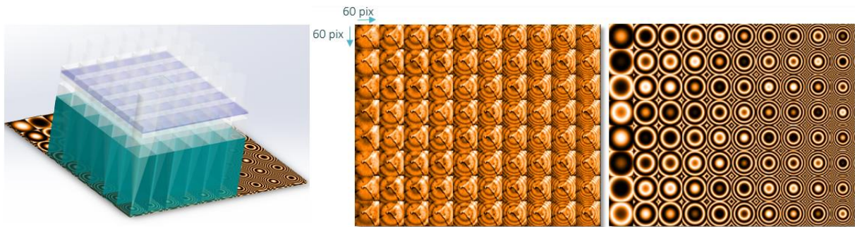
Figure 1. Left: Interferometer (micro-lenses + FP Silicon slides). Middle: Multiple small images of field of view modulated by Fabry-Perot rings on the detector. Right: monochromatic Fabry-Perot rings corresponding to selected OPD around maximum sensitivity detection of CO 2 concentration
