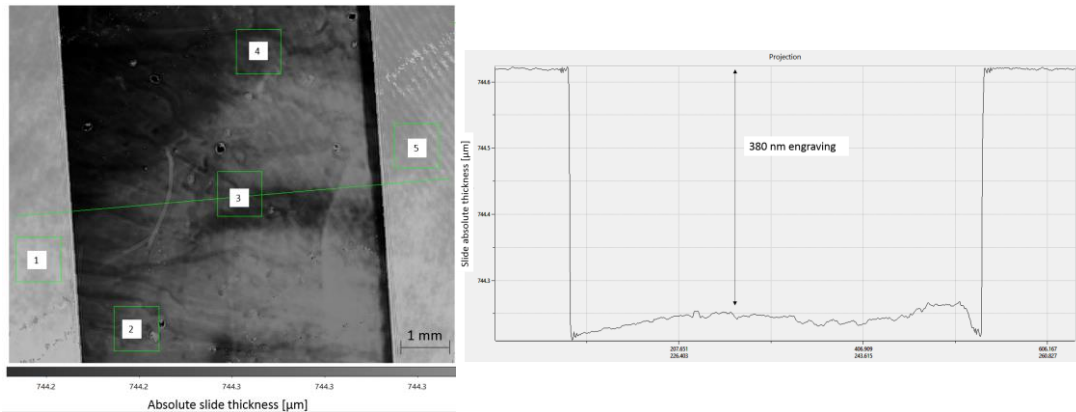
Figure 12. First engraved sample of silicon. Left: combined absolute thickness map. Right: profile of the absolute thickness map across the green line.
