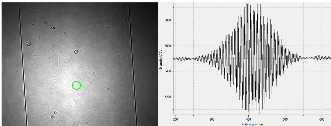
Figure 8 Left: raw image of the pupil intensity, for a given position of the delay line. The silicon plate we scan is 500 nm depth engraved in a rectangular area. The image shows the two diffracted parallel edges of this area. Right: extracted interferogram from the green-circled area, as a function of the position of the delay line device.
