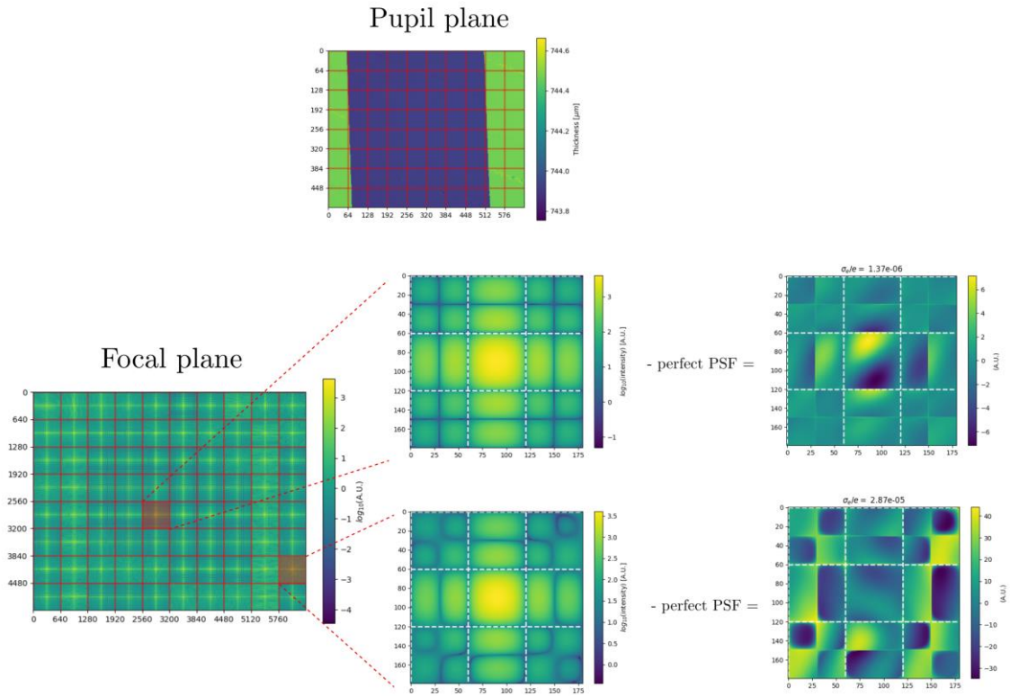
Figure 14. Example of calculated square microlens array PSF at detector level introduced by silicon slide inhomogeneities. Up: At pupil plane of second engraved sample of silicon slide used for
