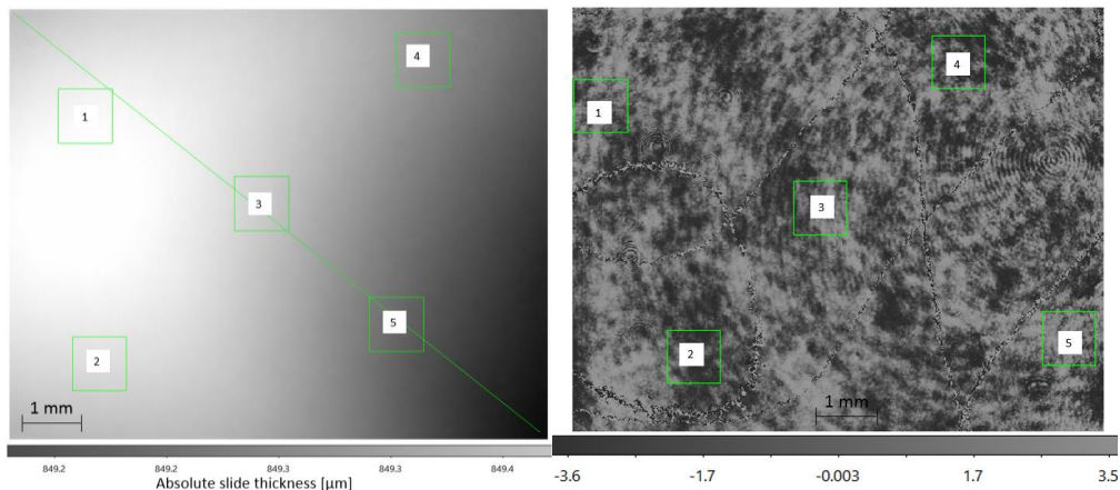
Figure 11. Thinned silicon sample. Left: combined absolute thickness map. Right: fine OPD variations.
