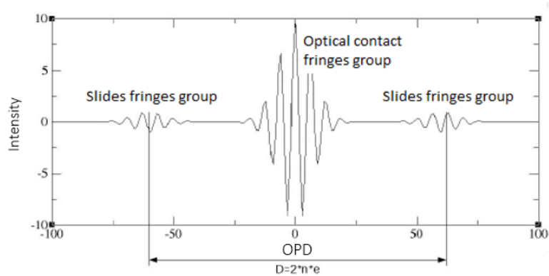
Figure 7. Interferogram obtained after moving the delay line to the position corresponding to the OPD introduced by silicon slides.
