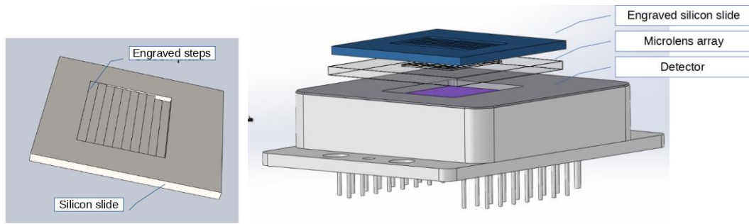
Figure 3. NanoCarb Engraved silicon slide is placed in front of microlens array. Each microlens sees a unique spaced Fabry-Perot which make an annealed Fabry-Perot figure over series thumbnail of field of view (see Figure 1).
