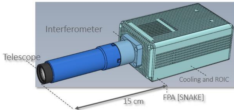
Figure 2. Schematics of NanoCarb infrared prototype with prefocal optics masking observed field of view to avoid thumbnail overlapping and adapting scale of field of view to ImSPOC sampling
