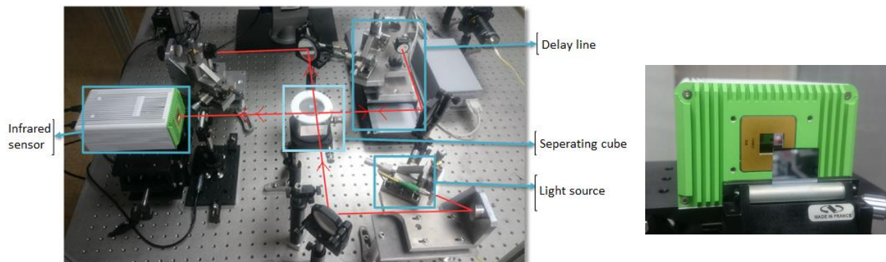
Figure 6. Left: OCT characterization bench. Right: Silicon slides placed in front of the infrared detector.
