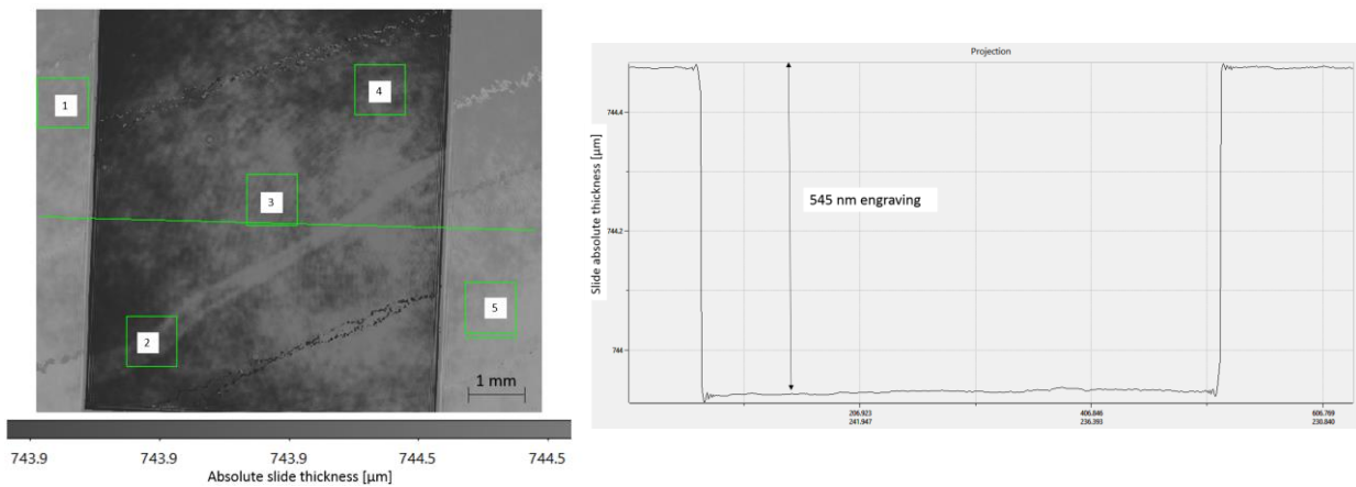
Figure 13 Second engraved sample of silicon. Left: combined absolute thickness map. Right: profile of the absolute thickness map across the green line.
