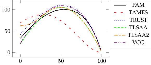
Fig. 5: Average Revenue as a function of the reserve price R
