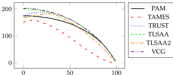
Fig. 6: Average social welfare as a function of the reserve price R
