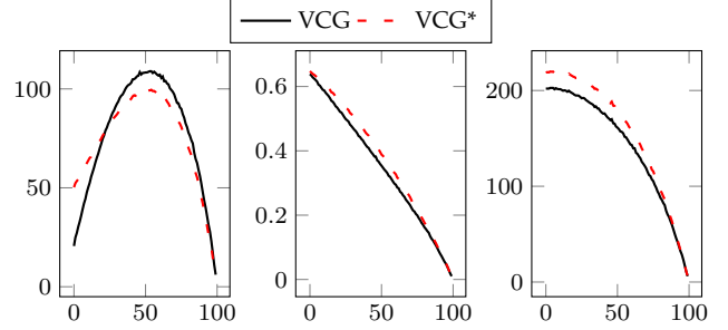
Fig. 8: Average revenue (left), fairness (center) and social welfare (right) as a function of the reserve price.
