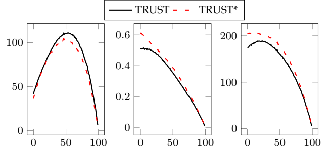
Fig. 7: Average revenue (left), fairness (center) and social welfare as a function of the reserve price.
