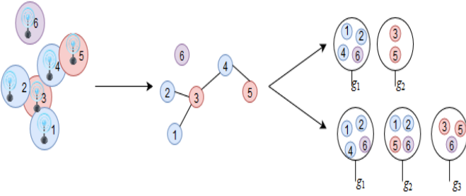
Fig. 3: Some base stations with their coverage areas (left), the corresponding interference graph (center), and two possible group configurations (right).
