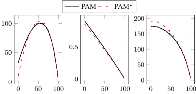
Fig. 9: Average revenue (left), fairness (center) and social welfare (right) as a function of the reserve price.
