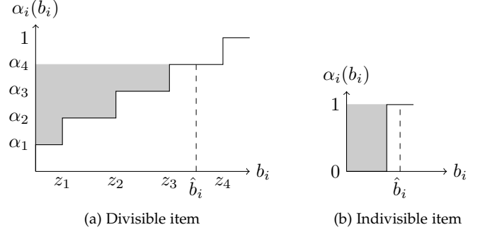
Fig. 2: Some piecewise constant monotone allocation curves (solid curves). The grey area represents the price paid when the bid b_i has value \hat{b}_i .
