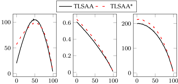
Fig. 10: Average revenue (left), fairness (center) and social welfare (right) as a function of the reserve price.
